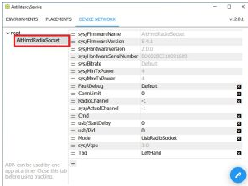
Fig. 5. Universal Radio Socket in the Device Tree
