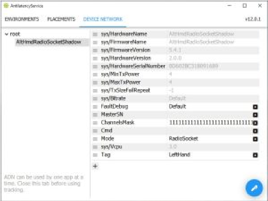
Fig. 4. The appearance of Universal Radio Socket as AltHmdRadioSocket and AltHmdRadioSocketShadow
