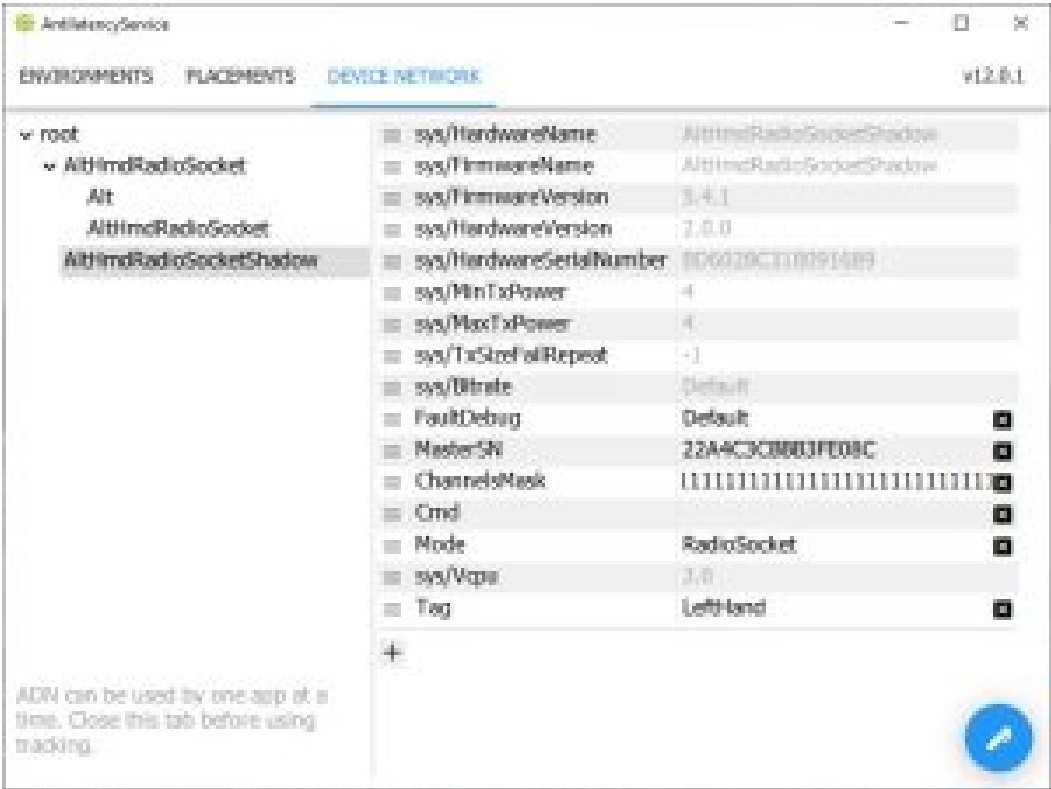
Fig. 3. The appearance of Universal Radio Socket as AltHmdRadioSocketShadow
