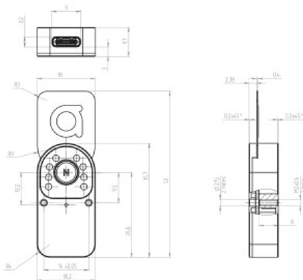
Fig. 1. Overall device dimensions
