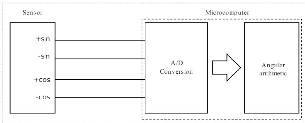
(ii) Configuration for A/D conversion after generating analog sin and cos signals
