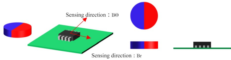
Fig.13 Layout of the magnet
