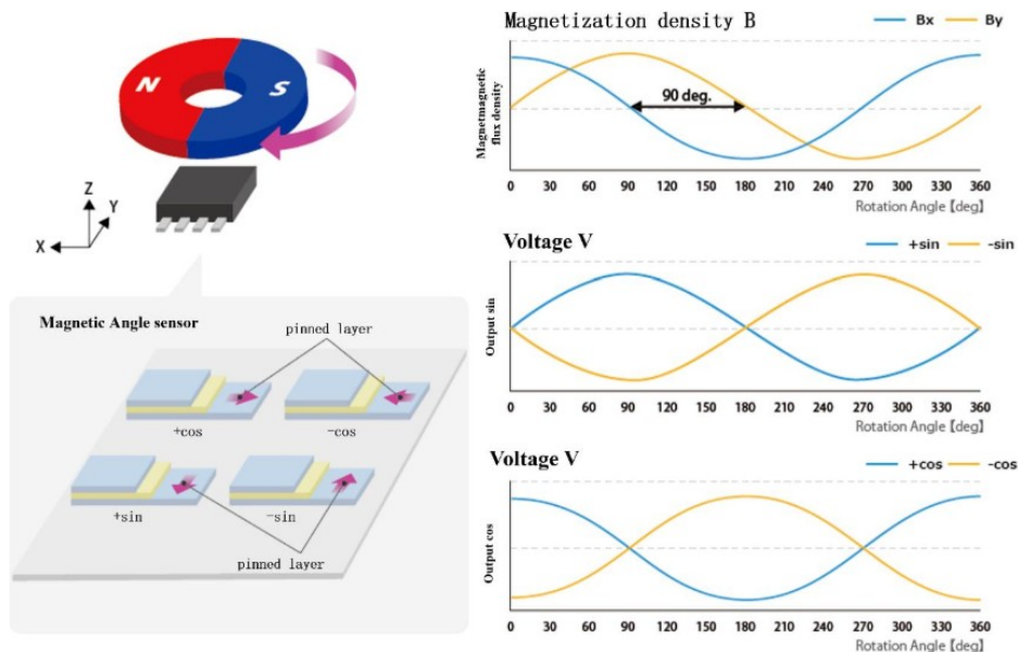
Fig.1 Output signal of magnetic angle sensor
