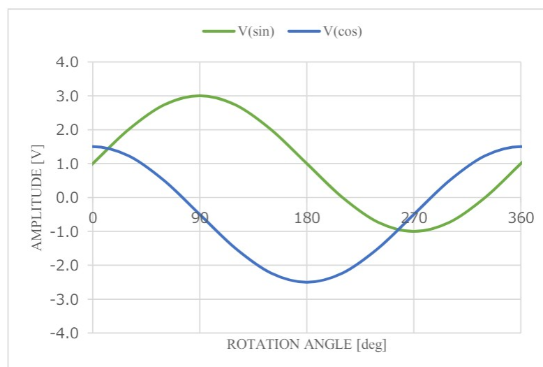
Fig.9 sin and cos signals
