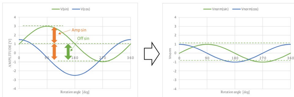
Fig.12 Normalization (Amplitude 1, Offset 0)
