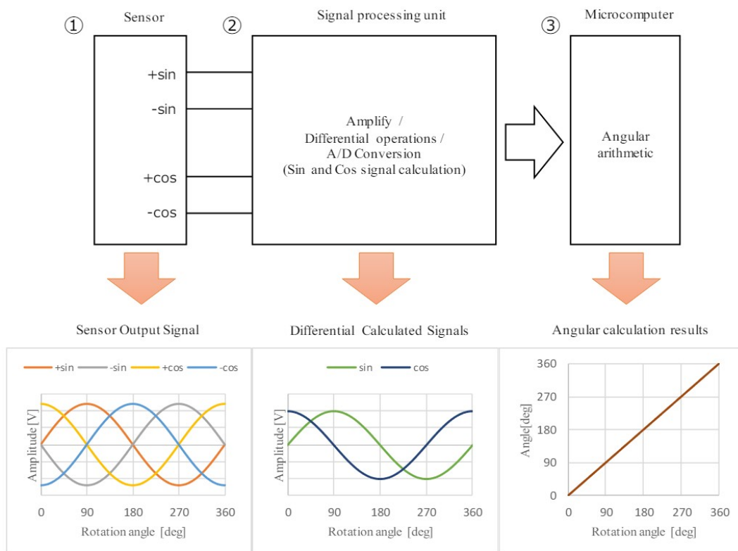
Fig.2 Angle calculation flow
