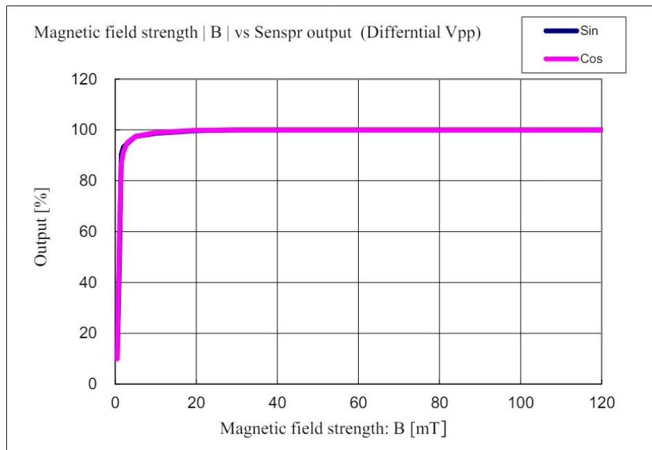
Fig.6 Sensor output character (@VDD 5V)
