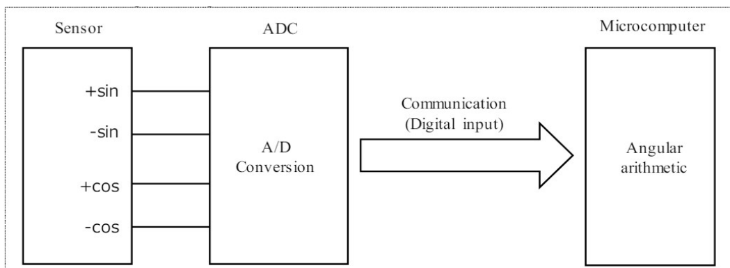
Fig.3 Examples for system structure
