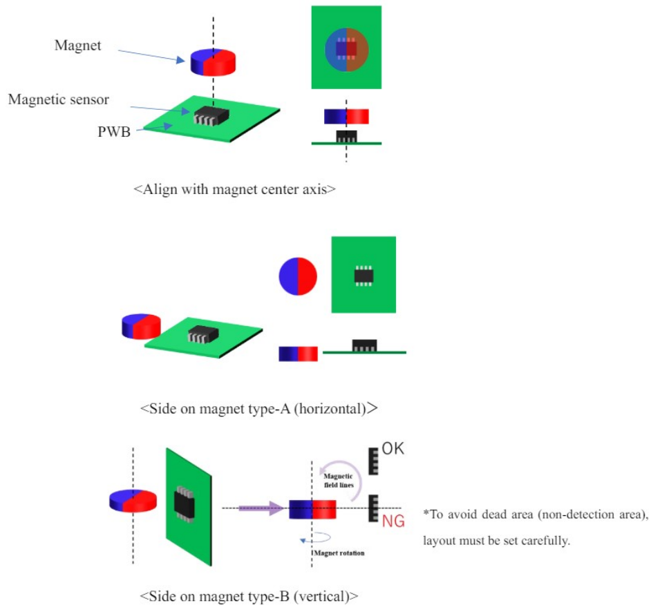
Fig.5 Layout of magnetic angle sensor
