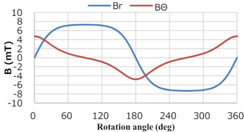
Fig. 14 Magnetic strength field near magnet (Br, Bθ)
