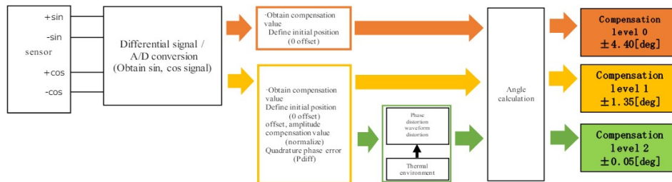
Fig.8 Compensation flow at desired level
