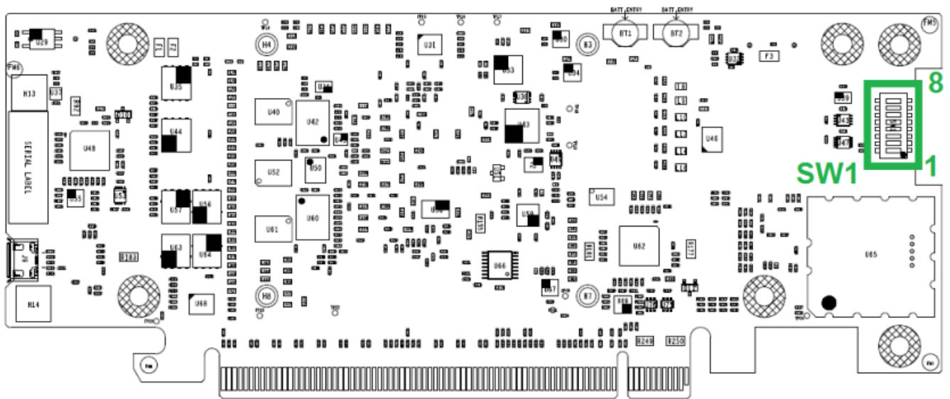
Figure 8 : Switches
