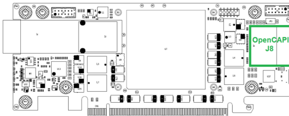
Figure 13 : OpenCAPI Location
