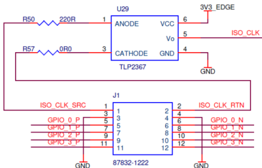
Figure 14 : GPIO Connector Schematic
