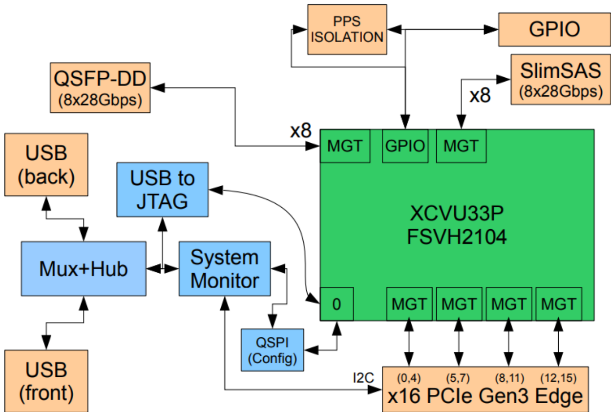
Figure 7 : ADM-PCIE-9H3 Block Diagram
