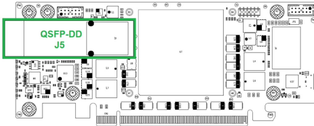
Figure 12 : QSFP-DD Location
