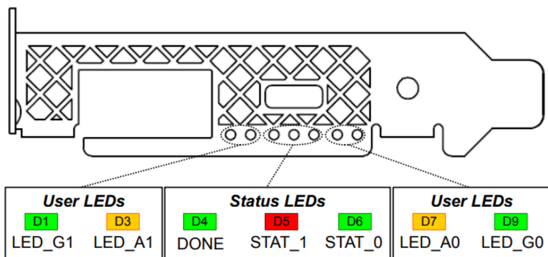
Figure 9 : Front Panel LEDs
