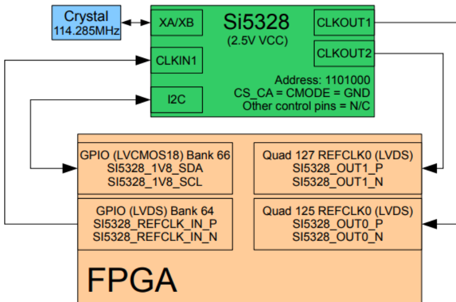
Figure 11 : Si5328 Block Diagram
