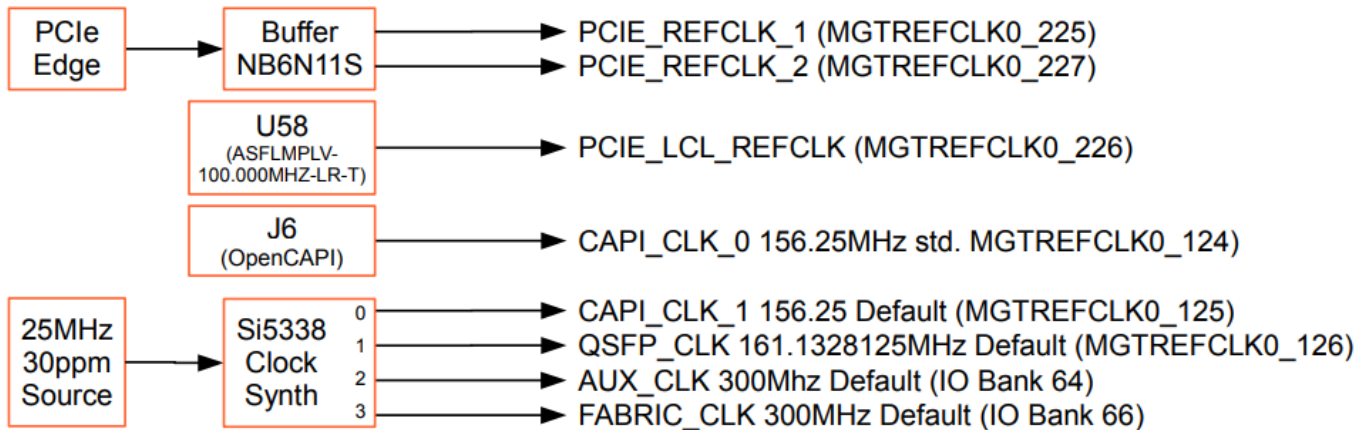
Figure 10 : Clock Topology
