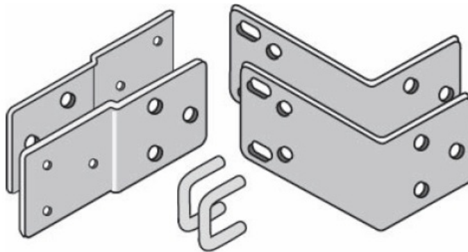
RKMT-J13 bracket kit for installing the GS970M/18 and GS970M/18PS Switches in an equipment rack.
