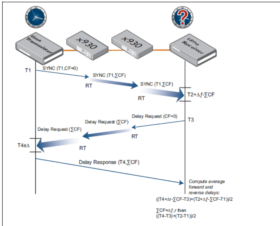
Figure 3: Overcoming errors using end-to-end Transparent Clock
