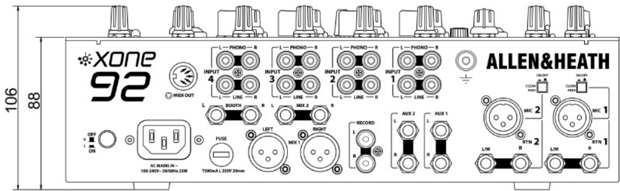
Front Panel
