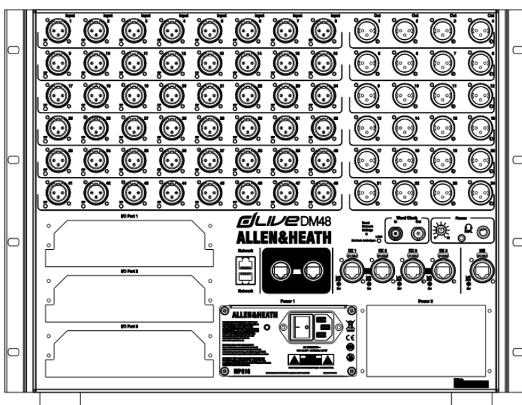
DM48 48 mic/line in 24 XLR out 8U
