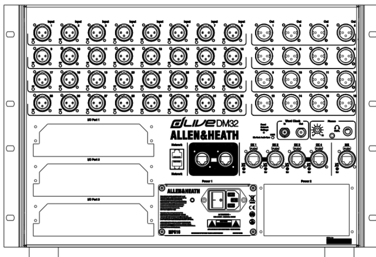
DM32 32 mic/line in 16 XLR out 7U
