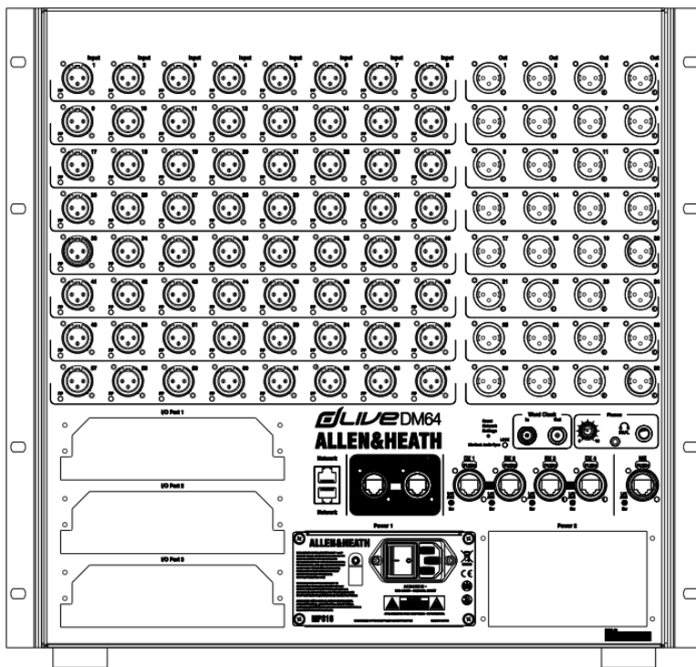
DM64 64 mic/line in 32 XLR out 10U
