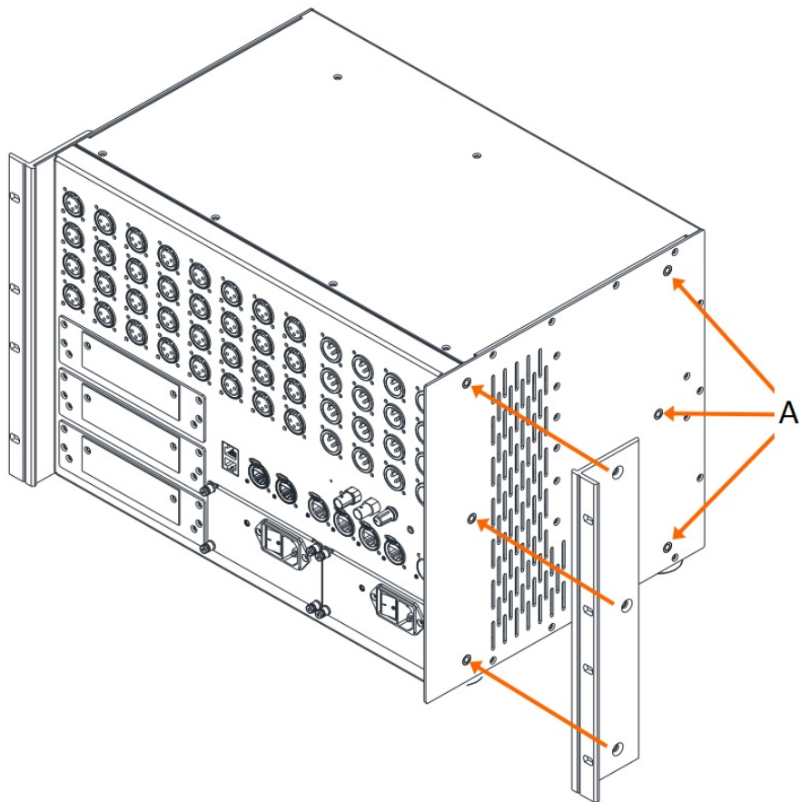
A Alternative front panel rack ear mounting
