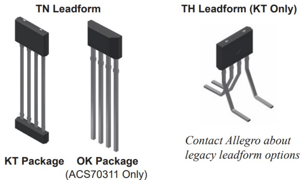
Figure 9: KT and OK Lead-forming Options
