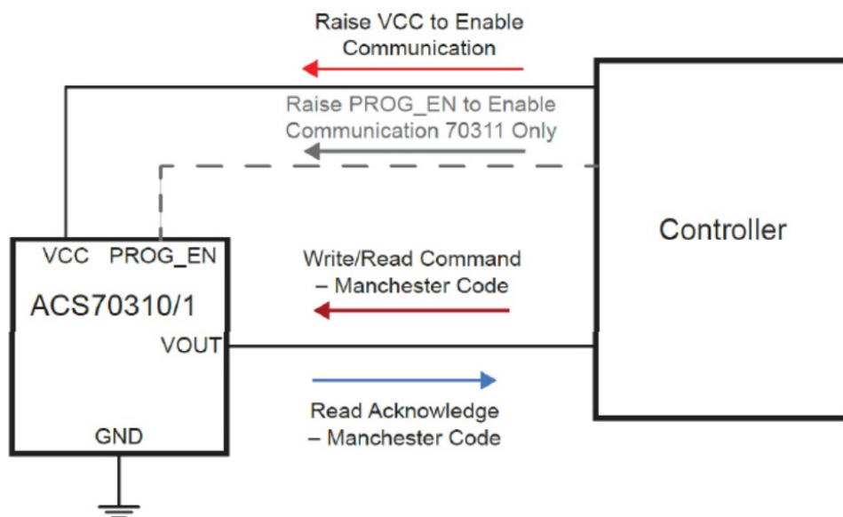
Figure 21: ACS70311 Programming Diagram
