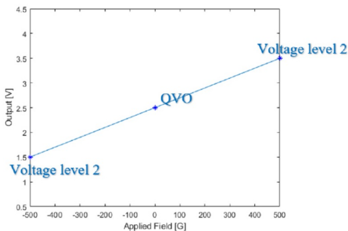
Figure 26: Calculating sensitivity using two known points
