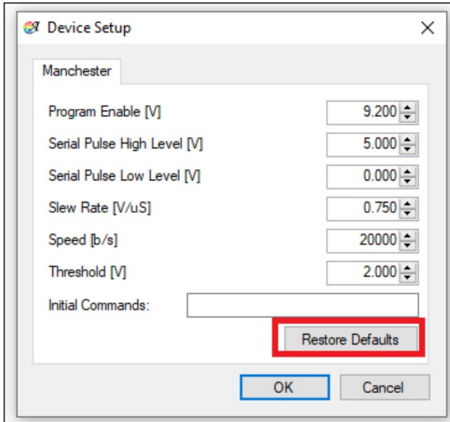
Figure 20: “Device Setup” menu defaults
