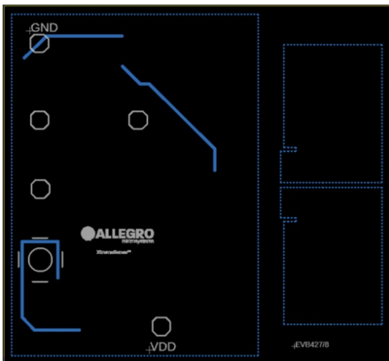
Figure 5: Bottom Layer
