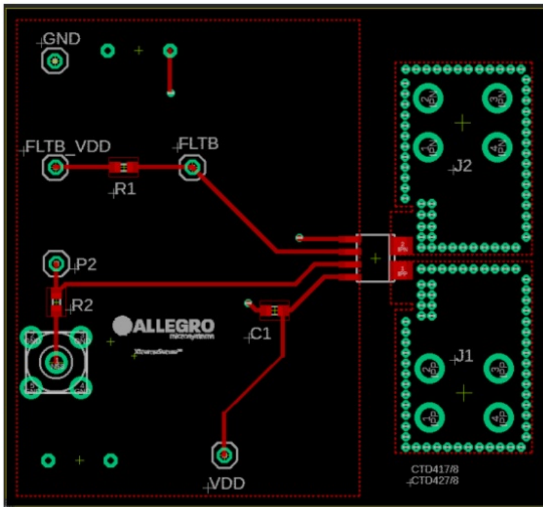
Figure 4: Top Layer
