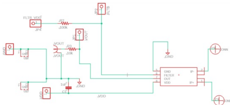
Figure 3: CT418-50AC Evaluation Board Schematic
