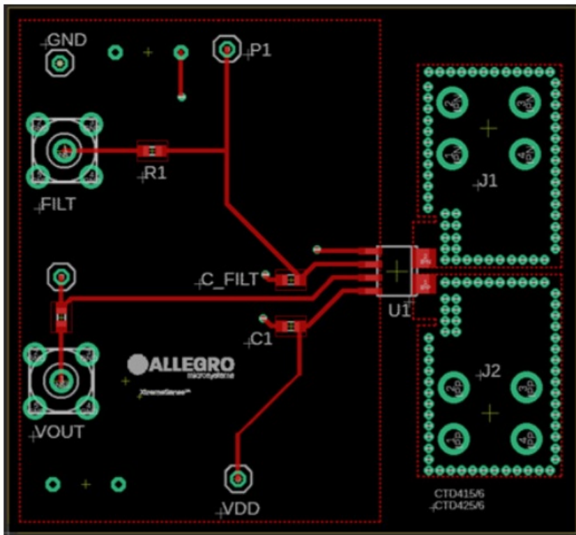
Figure 4: Top Layer
