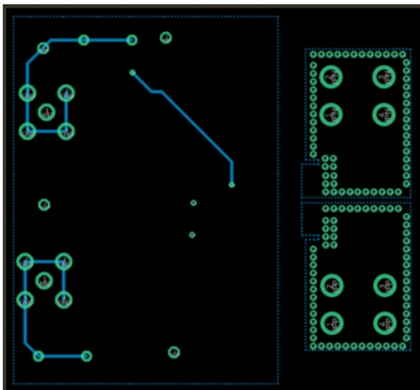
Figure 5: Bottom Layer
