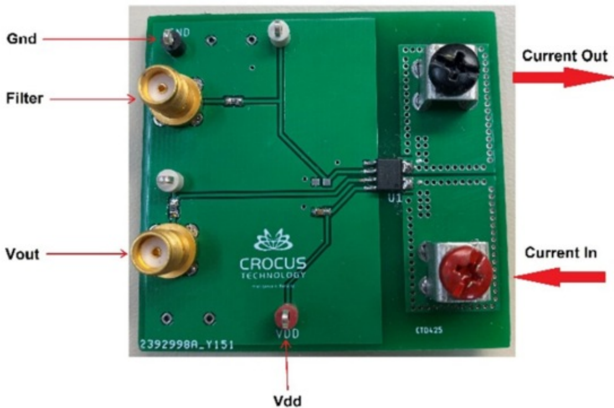
Figure 2: CT416-20AC Evaluation Board
