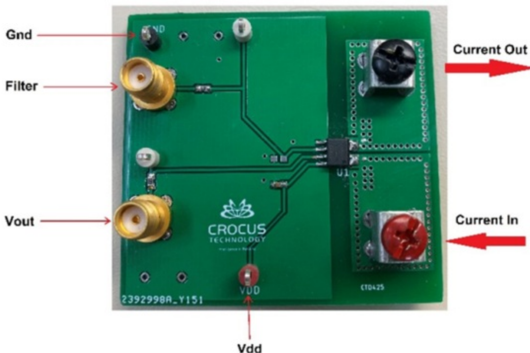
Figure 1: CT416-20AC Evaluation Board
