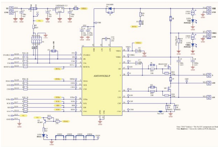
Figure 2: AMT49502KLP SMT Demo Board Schematic (1 of 2)
