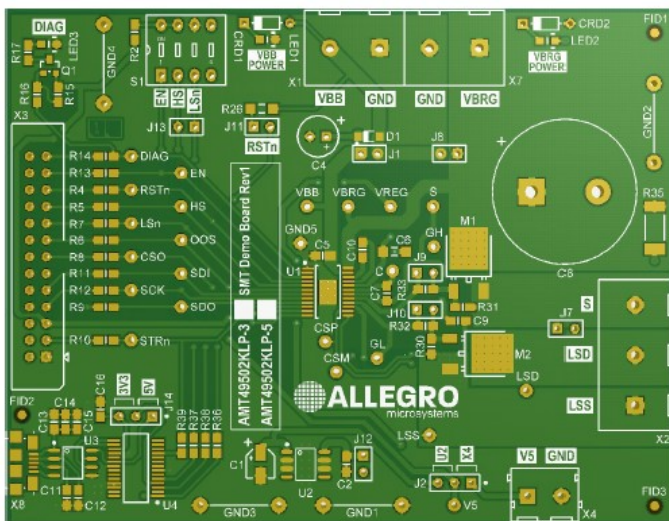
Figure 1: AMT49502 Demo Board
