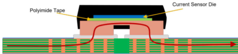
Figure 4: Vias Under Copper Pads Example
