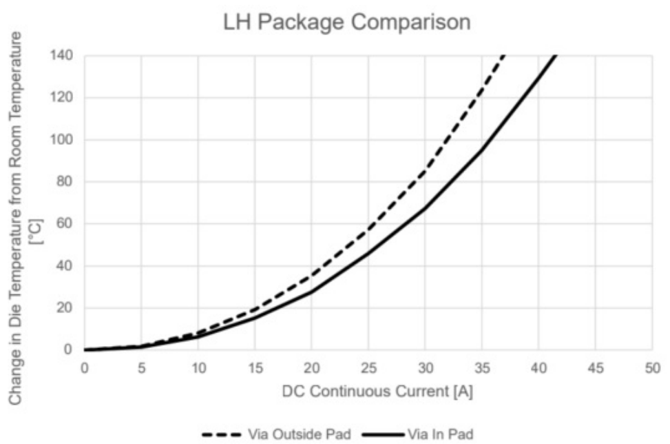
Figure 6: LH Package Comparison with and without In-Pad Vias
