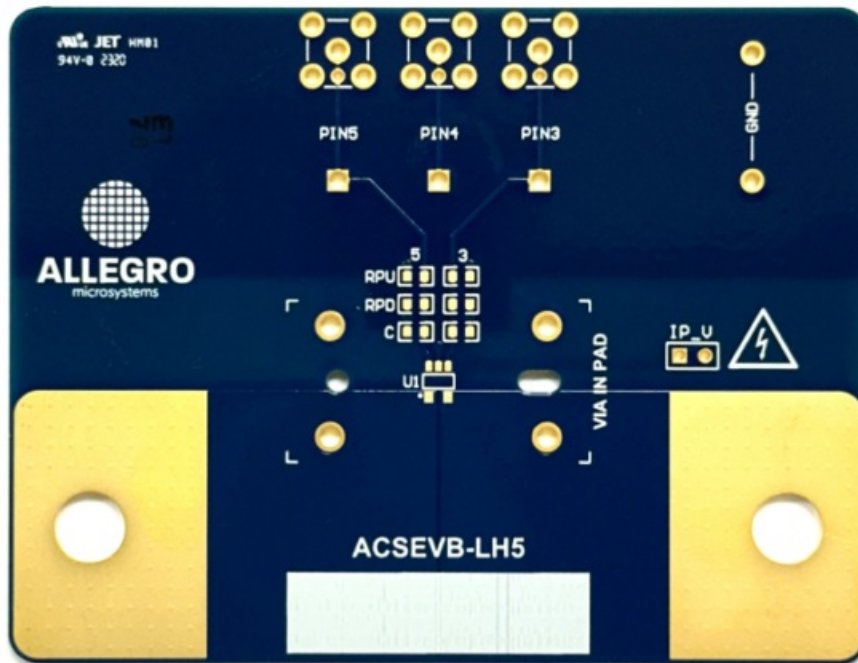
Figure 1: LH Bare Evaluation Board
