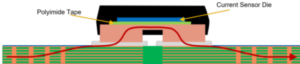
Figure 5: No Vias Under Copper Pads Example
