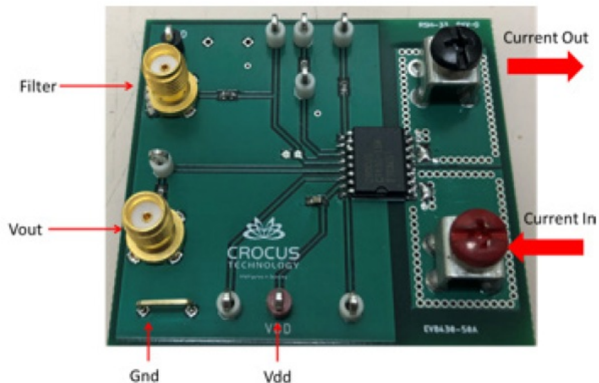
Figure 1: CT430-50AC Evaluation Board
