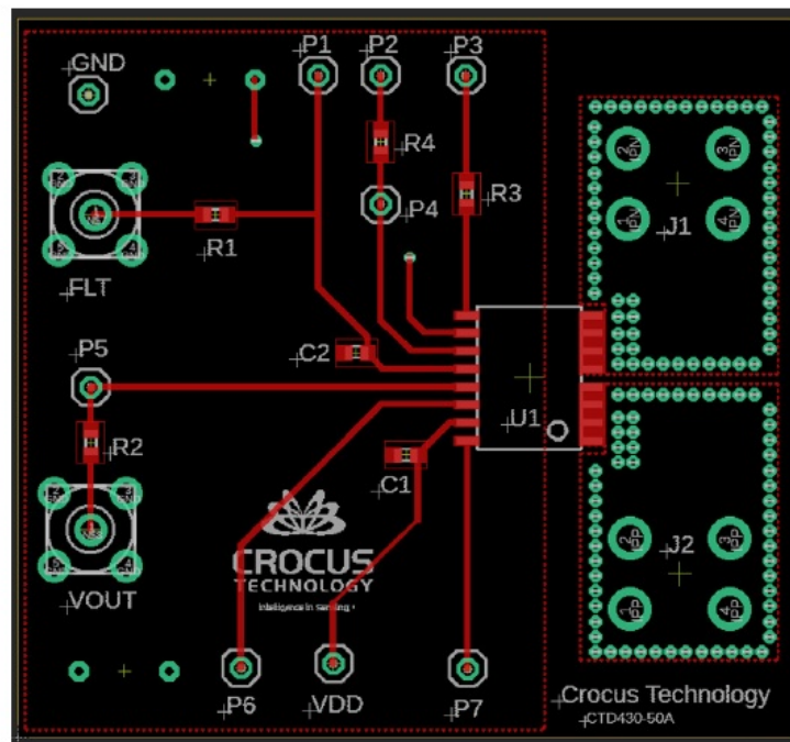
Figure 5: Top Layer
