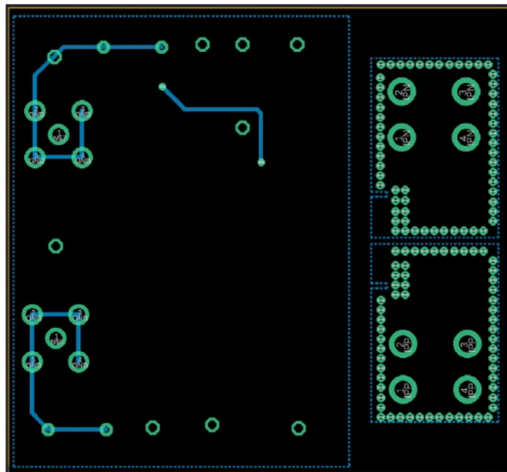
Figure 6: Bottom Layer
