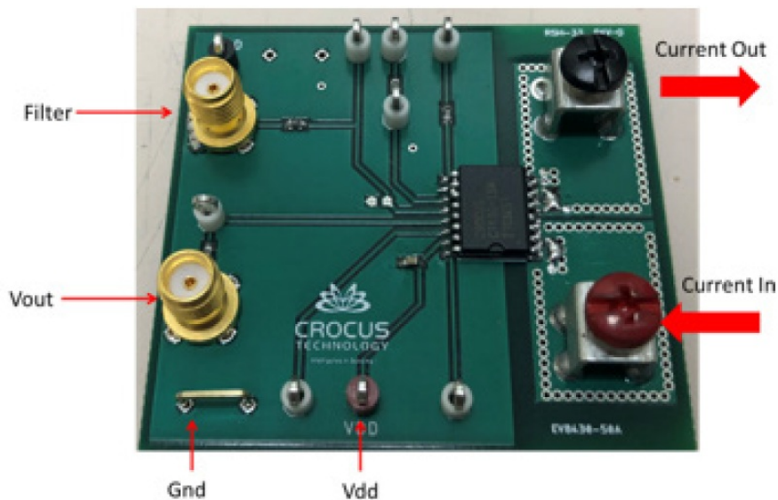
Figure 2: CT430-50AC Evaluation Board
