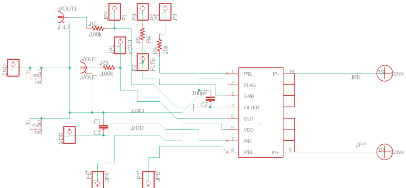
Figure 4: CT430-50AC Evaluation Board Schematic
