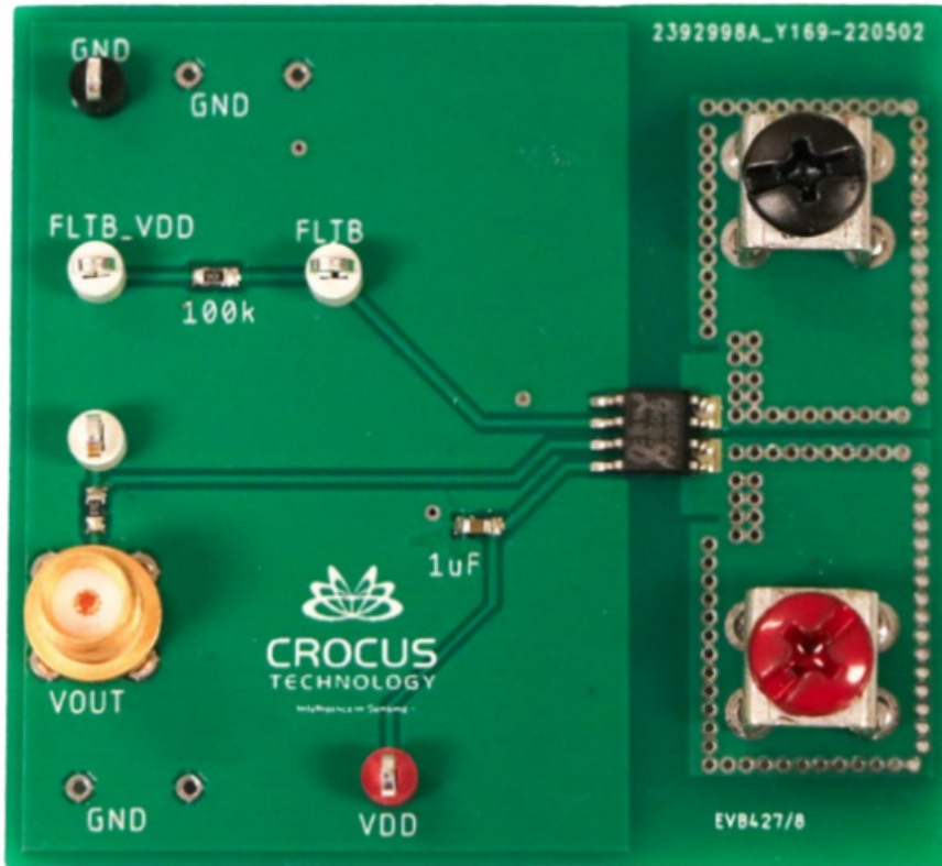
Figure 2: CT428-20AC Evaluation Board
