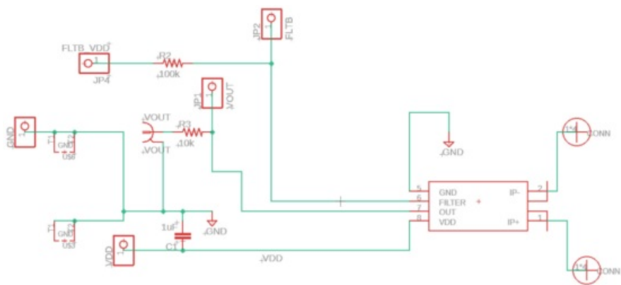
Figure 3: CT428-20AC Evaluation Board Schematic
