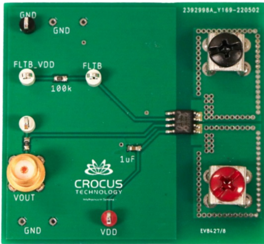
Figure 1: CT428-20AC Evaluation Board
