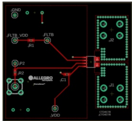
Figure 4: Top Layer
