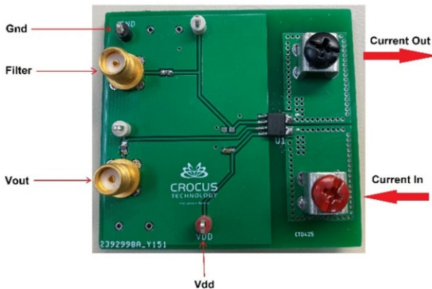
Figure 1: CT426-50AC Evaluation Board
