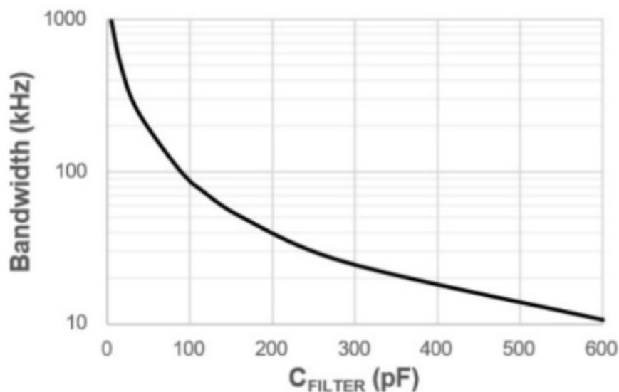
Figure 3: C_{\text{FILTER}} (pF) vs. 3 dB Cutoff Frequency (kHz)
