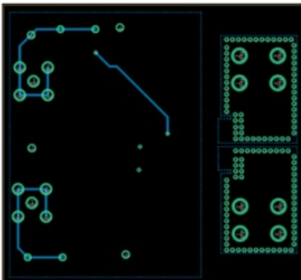
Figure 6: Bottom Layer
