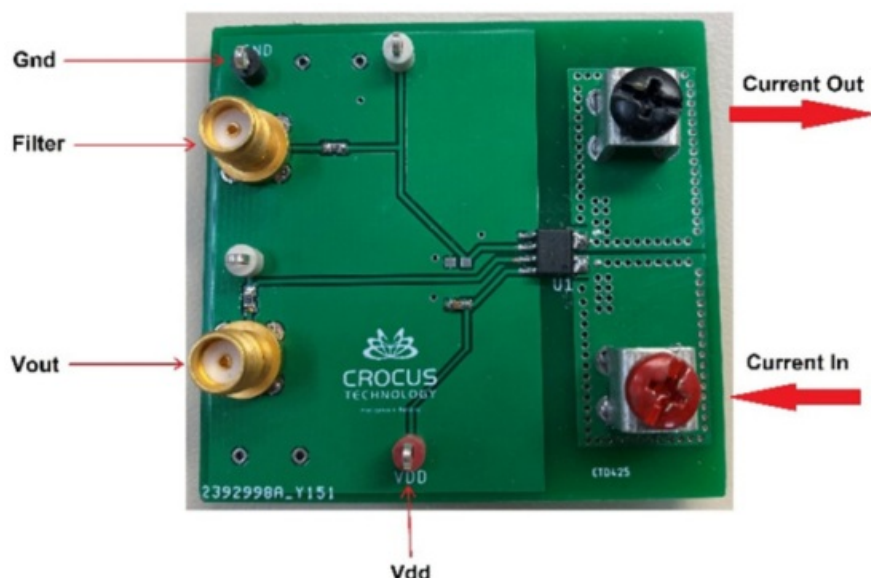
Figure 2: CT426-50AC Evaluation Board
