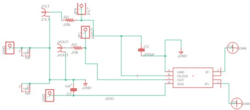
Figure 4: CT426-50AC Evaluation Board Schematic
