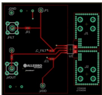
Figure 5: Top Layer
