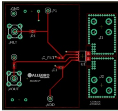
Figure 5: Top Layer
