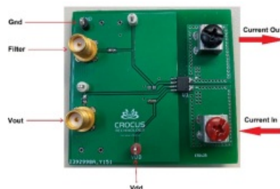
Figure 1: CT425-20AC Evaluation Board
