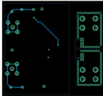
Figure 6: Bottom Layer
