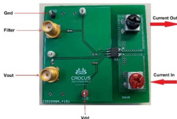
Figure 2: CT425-20AC Evaluation Board
