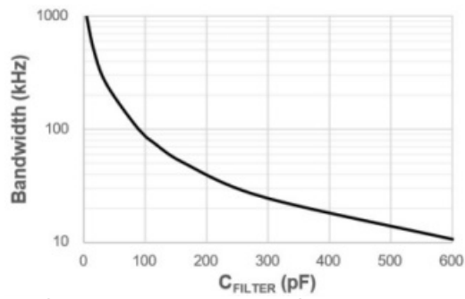
Figure 3: C_FILTER (pF) vs. 3 dB Cutoff Frequency (kHz)
