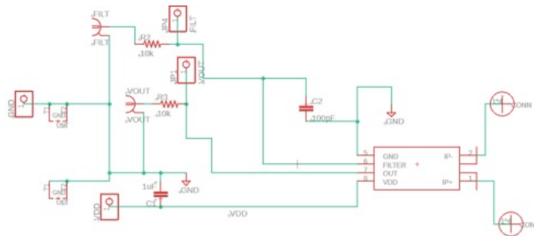
Figure 4: CT425-20AC Evaluation Board Schematic
