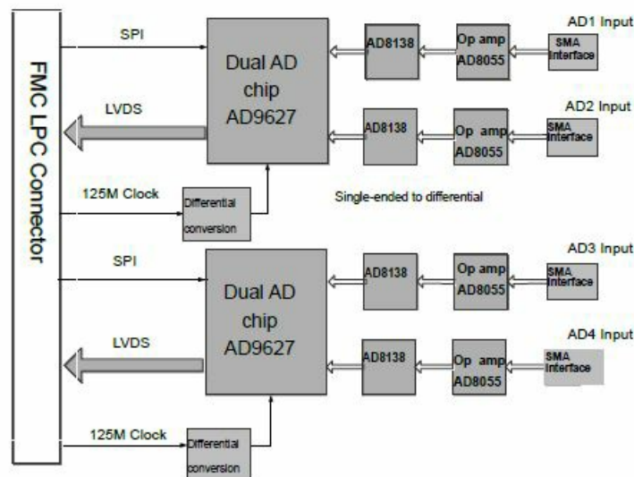
Figure 2-1: FL9627 Module Block Diagram For the circuit design of the AD9627, please refer to the chip manual of the AD9267.
