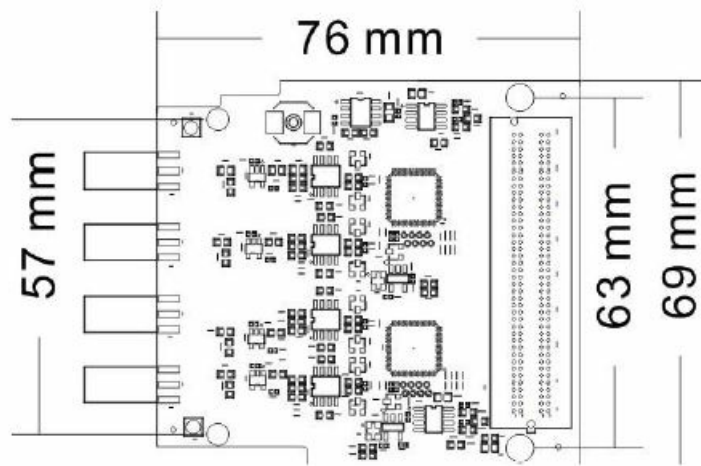
Figure 1-2: FL9627 FMC 4-channel High Speed AD Module Size Dimension
