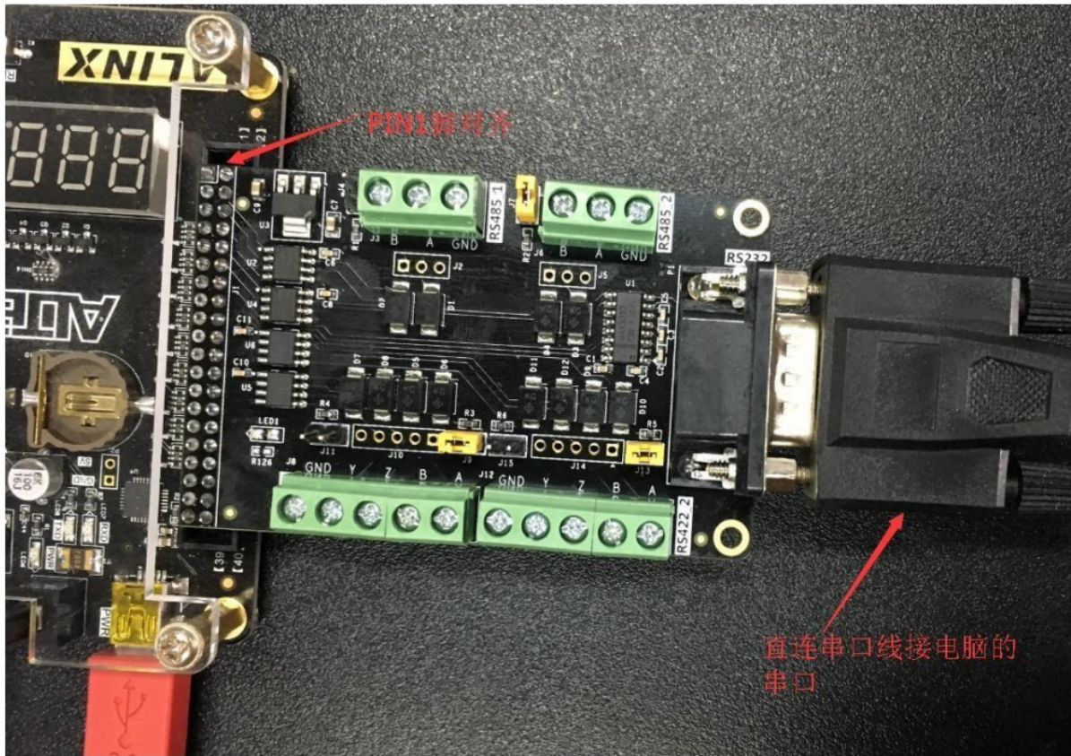
Figure 3-2: Hardware Connection
