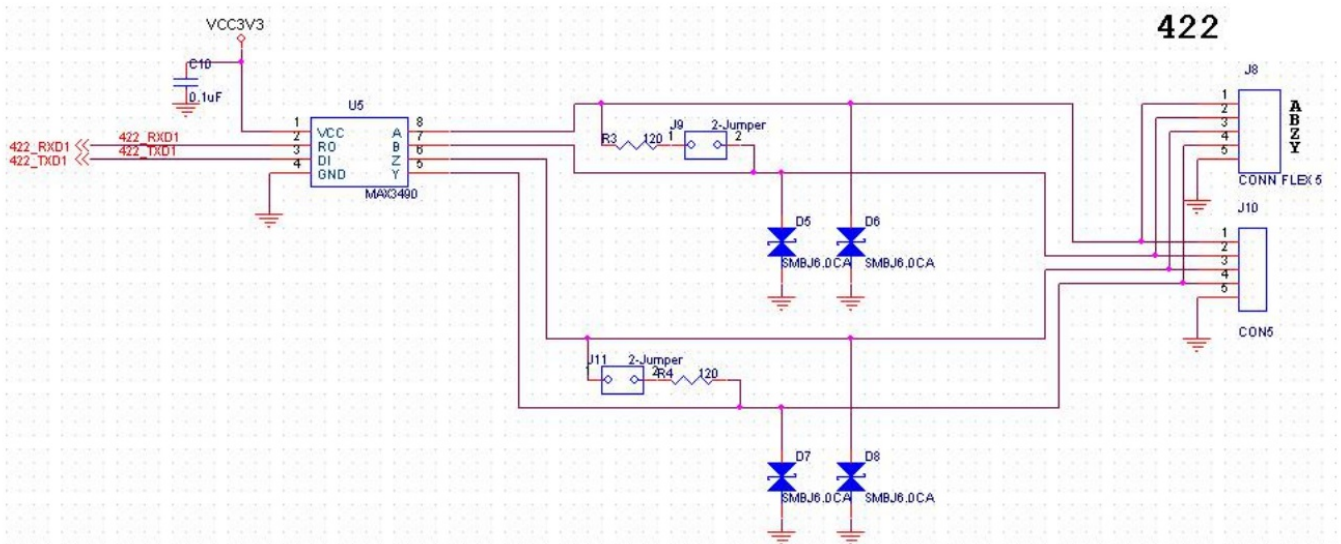
Figure 2-3: The RS422 Circuit Design
