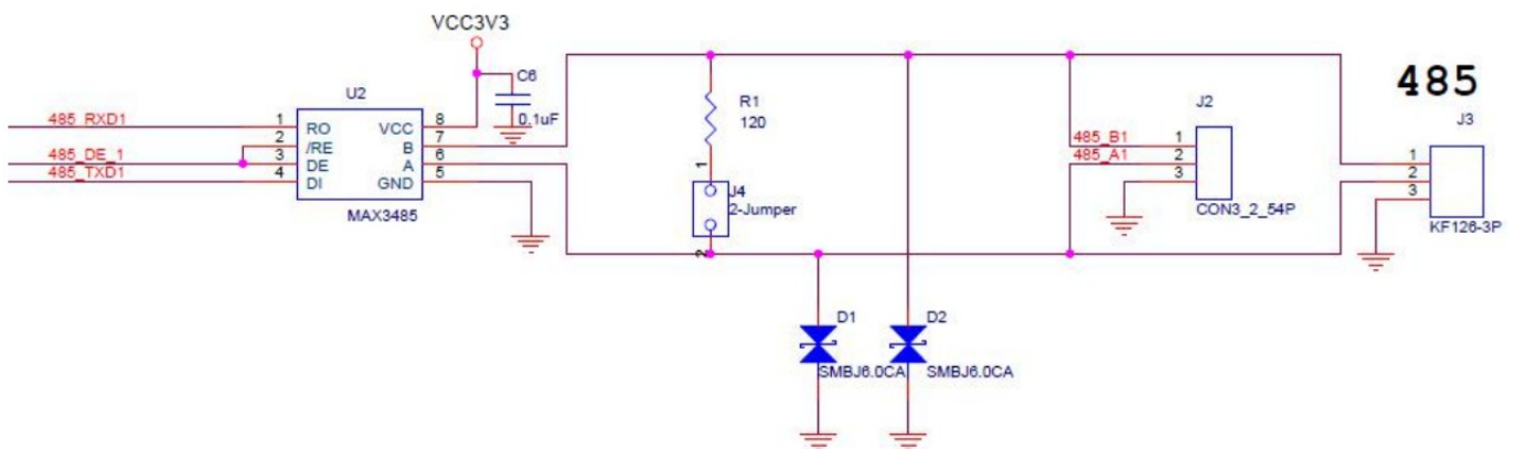
Figure 2-2: The RS485 Circuit Design
