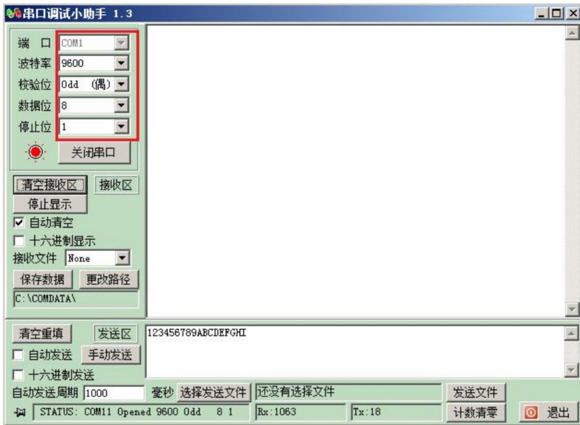
Figure 3-3: The Specific Configuration of Serial Debugging Assistant
