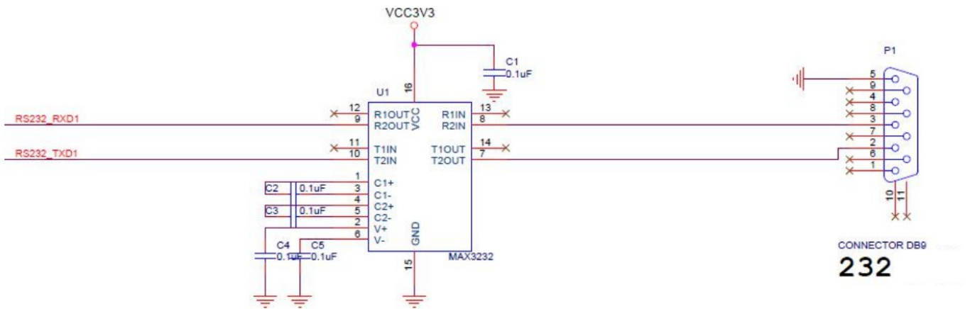
Figure 2-1: The RS232 Circuit Design
