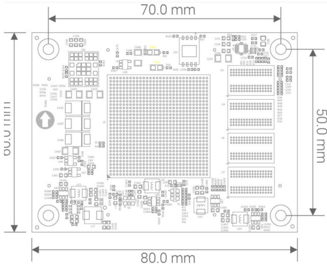
Figure 8-1: Top View
