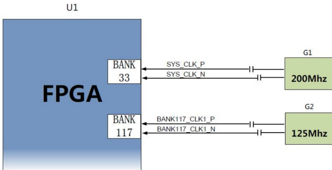
Figure 5-1: Core Board Clock Source
