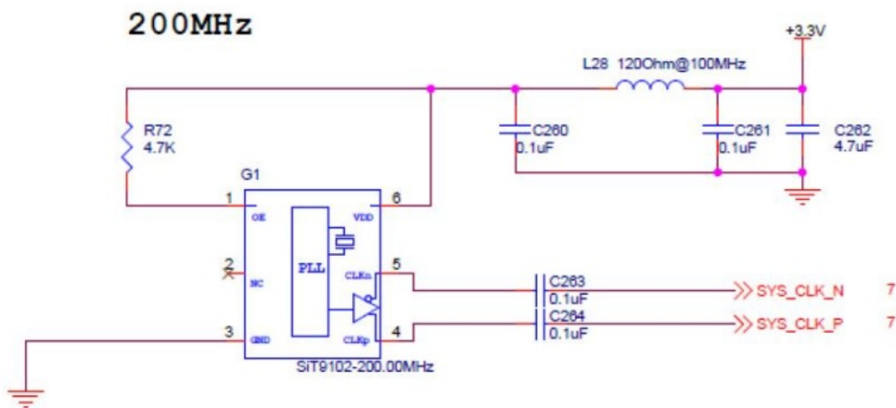
Figure 5-2: System clock source
