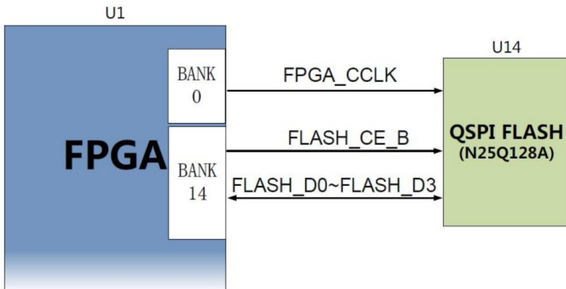
Figure 4-1: QSPI Flash Schematic
