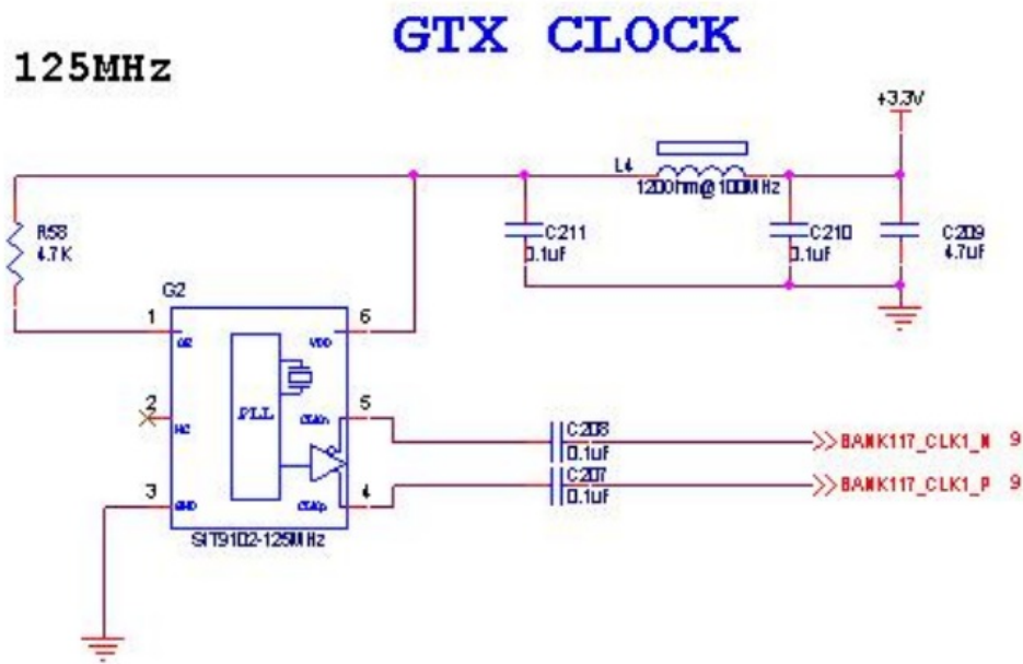
Figure 5-3: 125Mhz Active Differential Crystal Schematic
