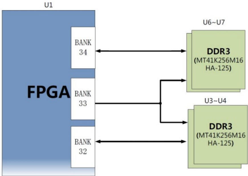
Figure 3-1: The DDR3 DRAM Schematic
