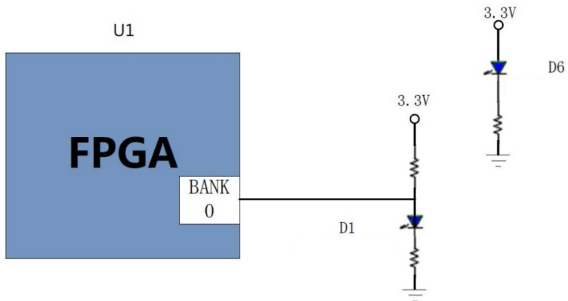
Figure 2-6-1: LED lights on core board Schematic
