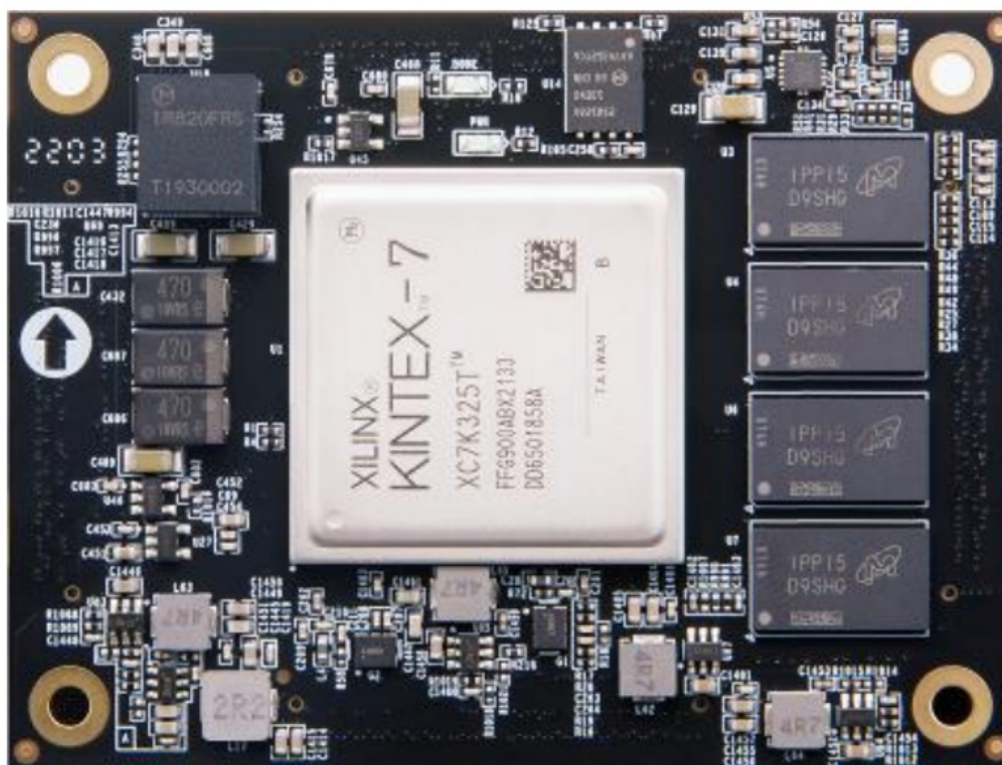
Figure 1-1: AC7K325B Core Board (Front View)
