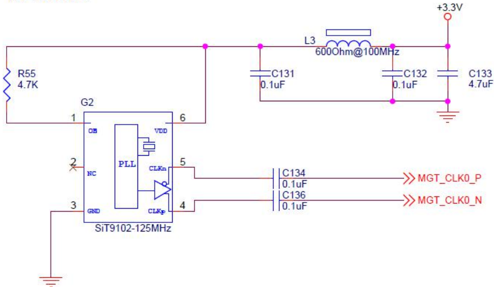
Figure 3-3: 125MHz Active Differential Crystal Schematic
