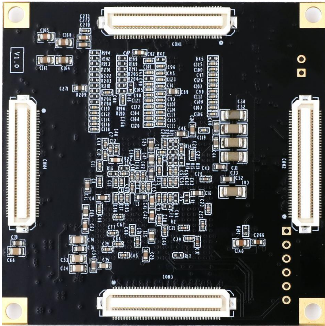
Figure 1-2: AC7A200 Core Board (Rear View)
