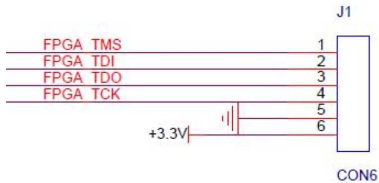
Figure 7-1: JTAG Interface Schematic
