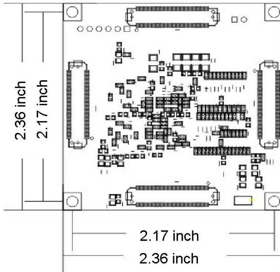
Figure 11-2: AC7A200 FPGA Core board (Bottom View)
