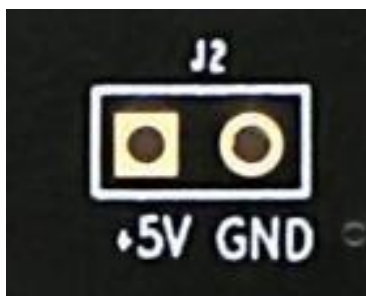
Figure 8-2 Power interface on the Core Board
