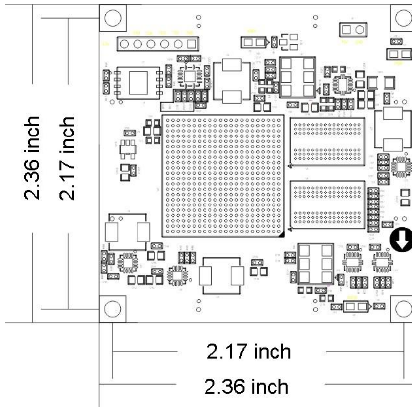
Figure 11-1: AC7A200 FPGA Core board (Top View)
