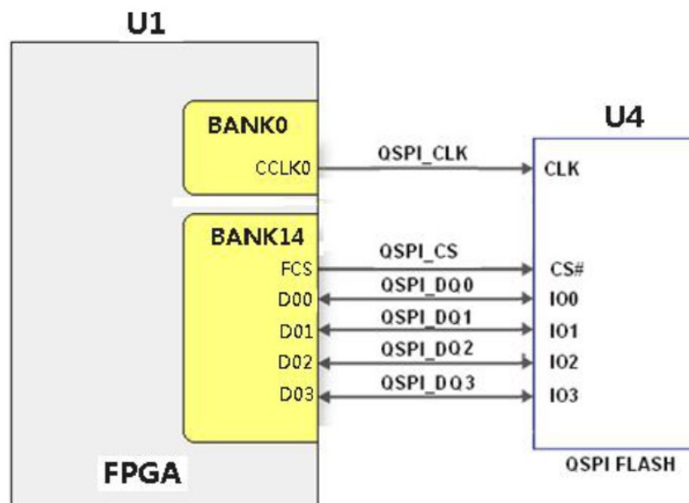
Figure 5-1: QSPI Flash Schematic
