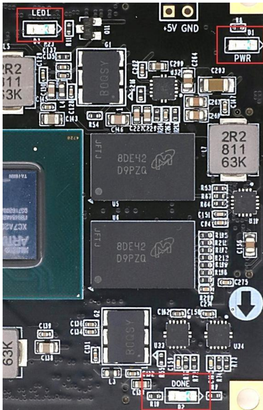
Figure 6-2: LED lights on the Core Board
