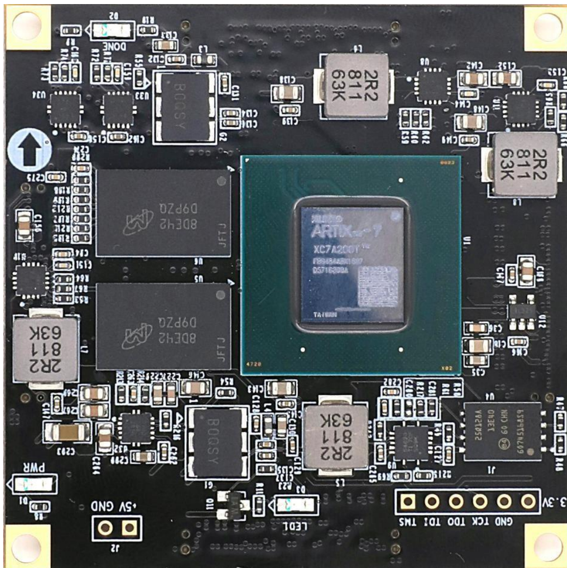
Figure 1-1: AC7A200 Core Board (Front View)
