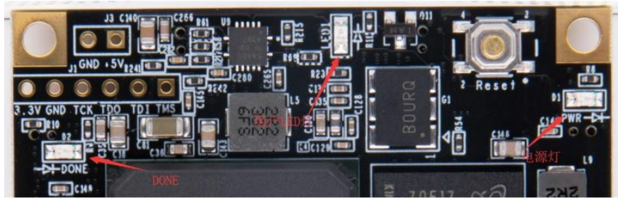
Figure 6-2: LED lights on the Core Board
