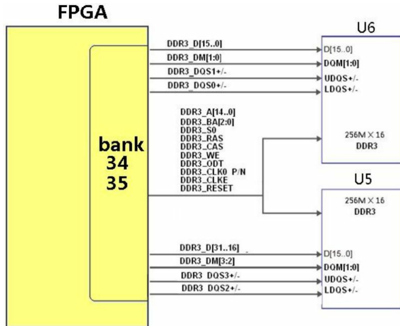
Figure 4-1: The DDR3 DRAM Schematic
