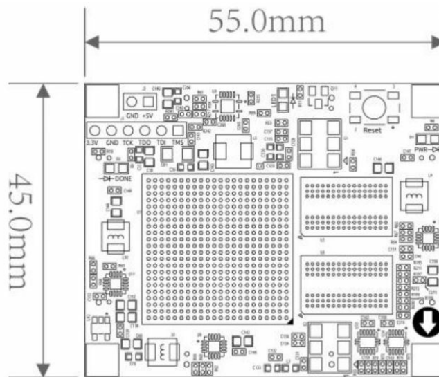
Figure 12-1: AC7200 FPGA Core board (Top view)
