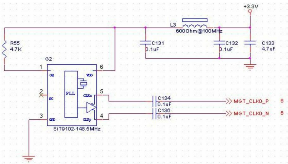
Figure 3-3: 148.5Mhz Active Differential Crystal Schematic
