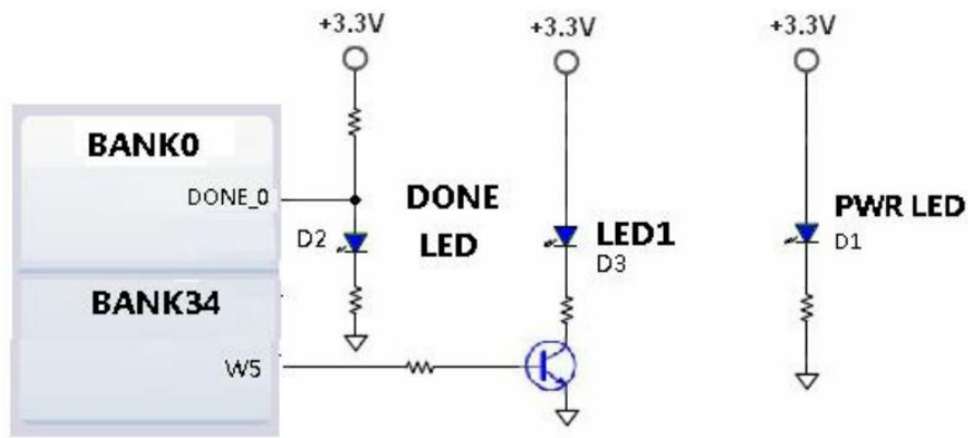
Figure 6-1: LED lights on core board Schematic
