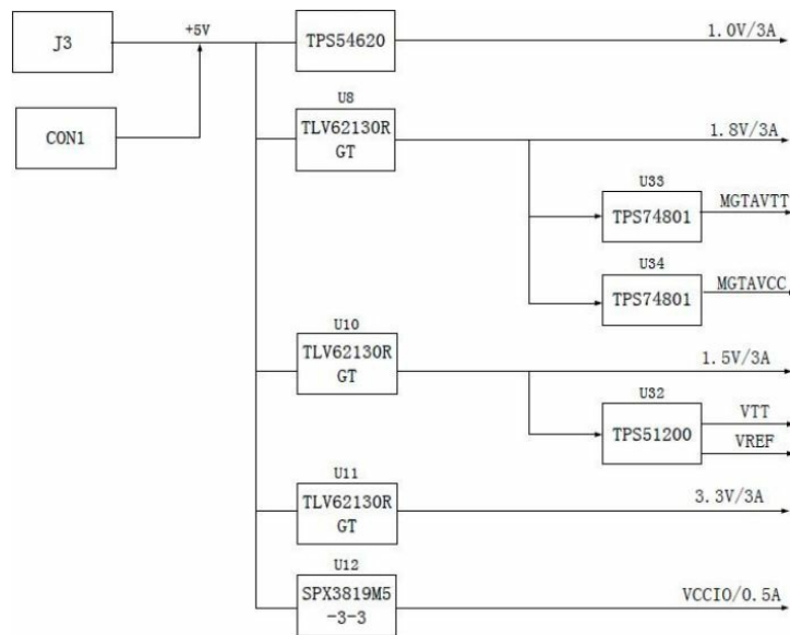
Figure 11-1: Power Supply on core board schematic
