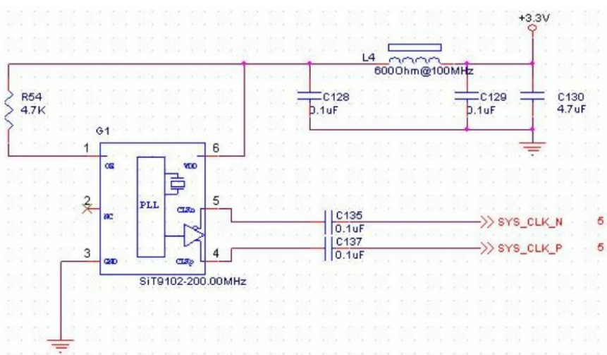
Figure 3-1: 200Mhz Active Differential Crystal Schematic
