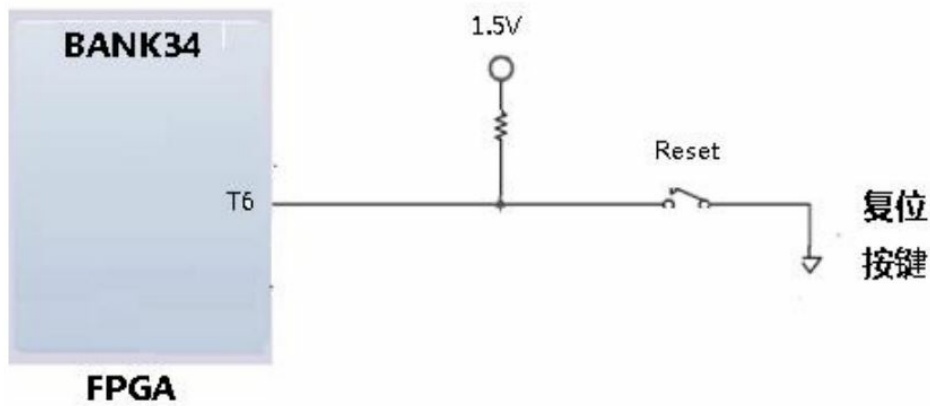
Figure 7-1: Reset Button Schematic
