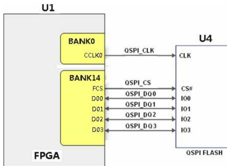
Figure 5-1: QSPI Flash Schematic
