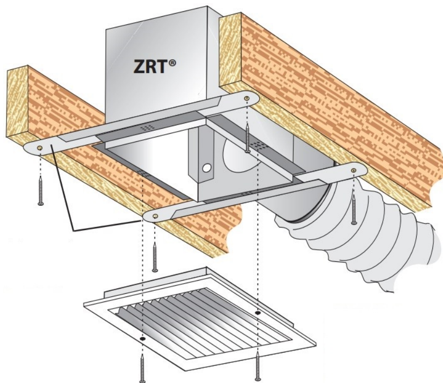
FIGURE 1 – MOUNTING
