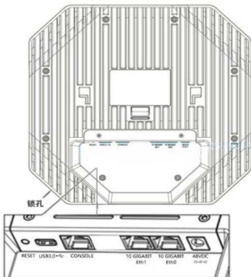
Figure 3: OAW-AP1351 Back View
