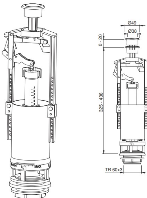
Flush valve with raised stop button
