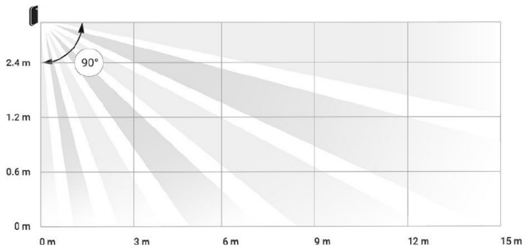
Horizontal and vertical detector's angles of view
