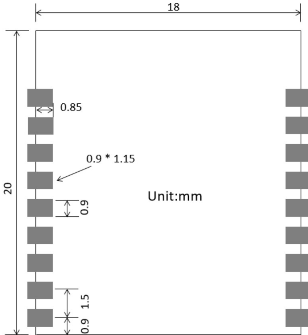
Fig. 3.3 PCB Layout for ESP-C20
