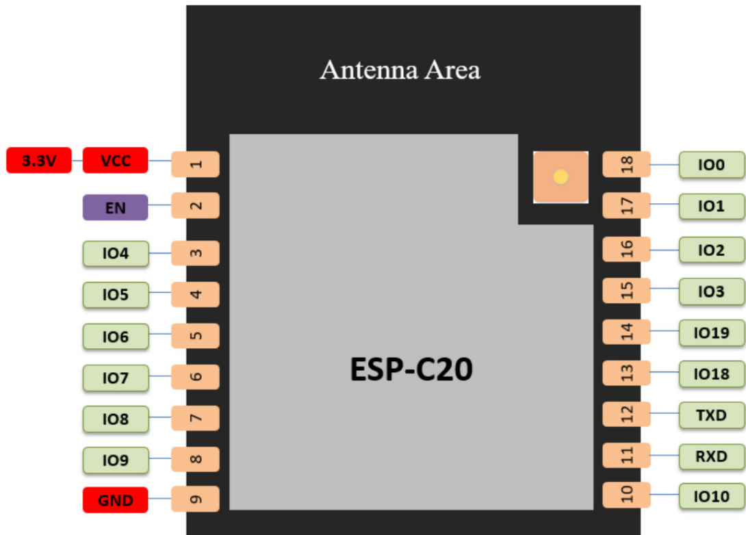
Fig.2.1 ESP-C20 Pins Definition
