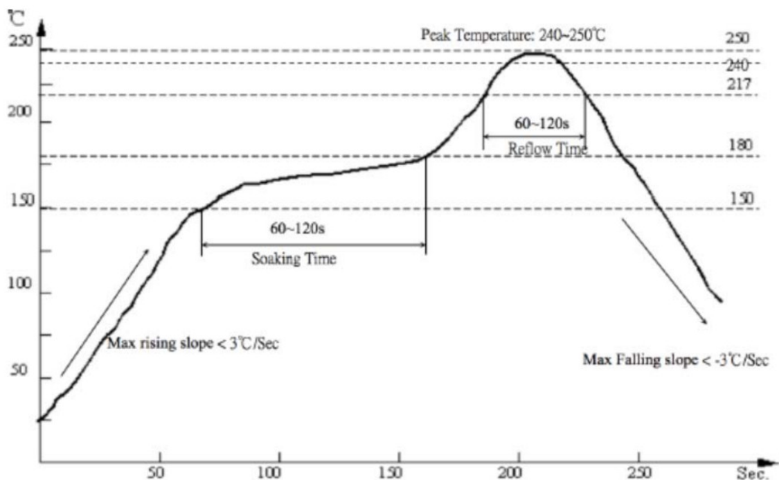
Fig.8.1 Recommended Reflow Profile
