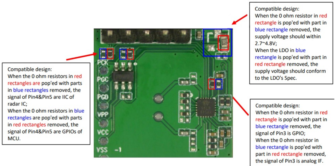
Plot. AT58L4LDB-2020 Module design detail
