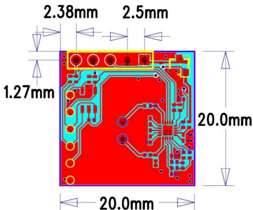
Plot. 3 AT58L4LDB-202 module dimension and connector location
