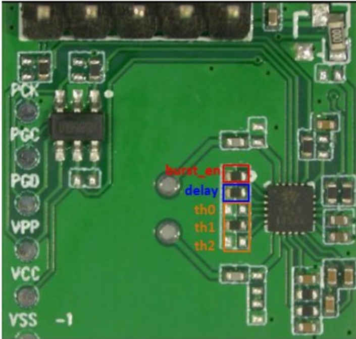
Plot. 4 on-board resistors setting illustration
