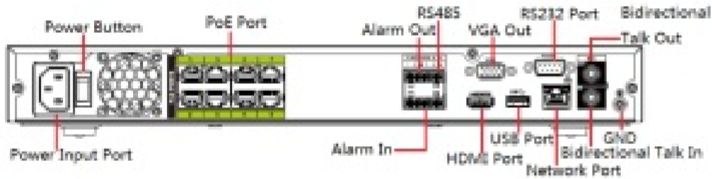
Figure 3-1 Connection sample
