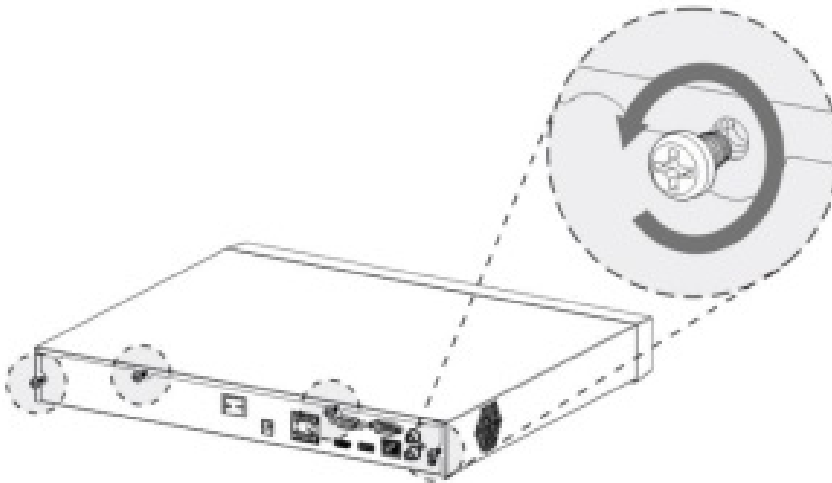
Figure 2-7 Installing HDD (1)
