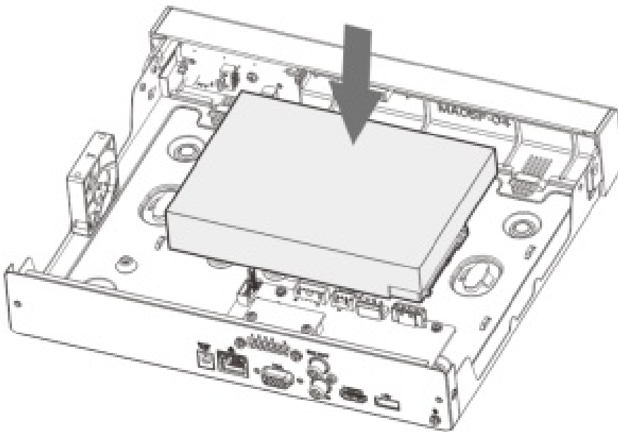
Figure 2-3 Installing HDD (3)
