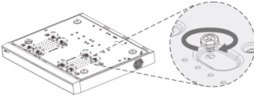
Figure 2-10 Installing HDD (4)
