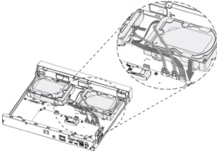
Figure 2-11 Installing HDD (5)
