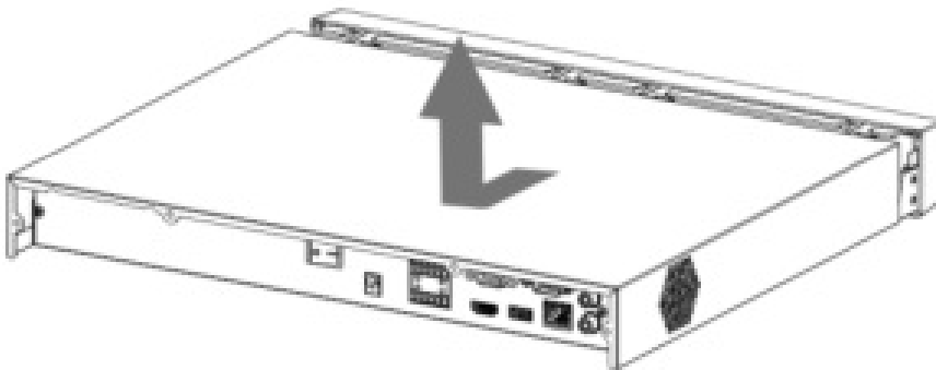
Figure 2-8 Installing HDD (2)
