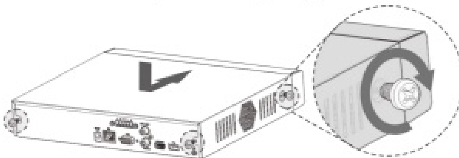
Figure 2-6 Installing HDD (6)
