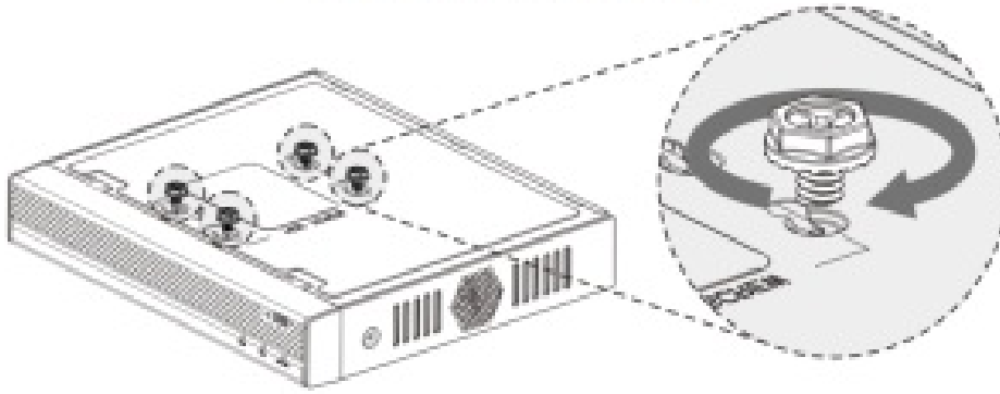
Figure 2-4 Installing HDD (4)
