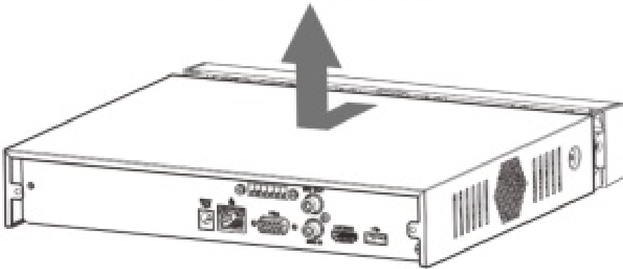
Figure 2-2 Installing HDD (2)
