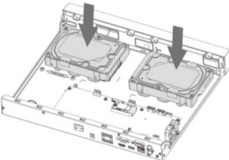
Figure 2-9 Installing HDD (3)
