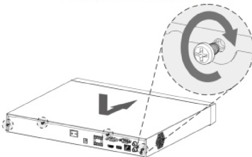
Figure 2-12 Installing HDD (6)
