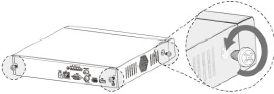
Figure 2-1 Installing HDD (1)
