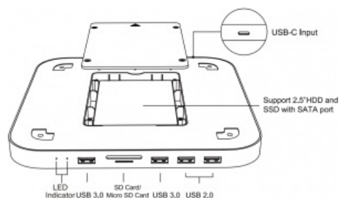
LED Indicator SD Card! Micro SD Card, USB 3.0, 2.0
