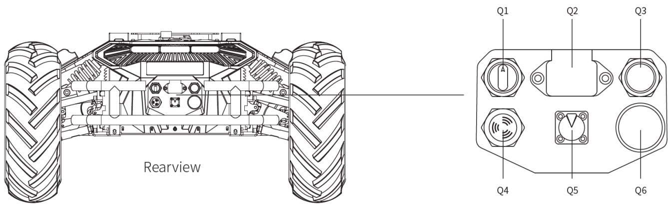
Figure 2.6 Rear View
