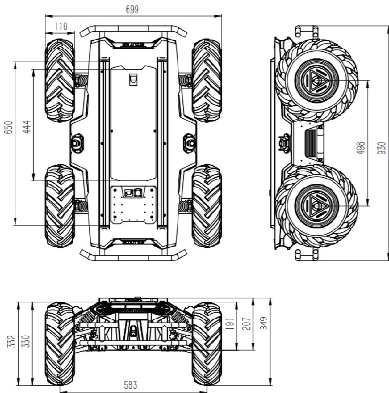
Illustration diagram of top extended support dimensions
