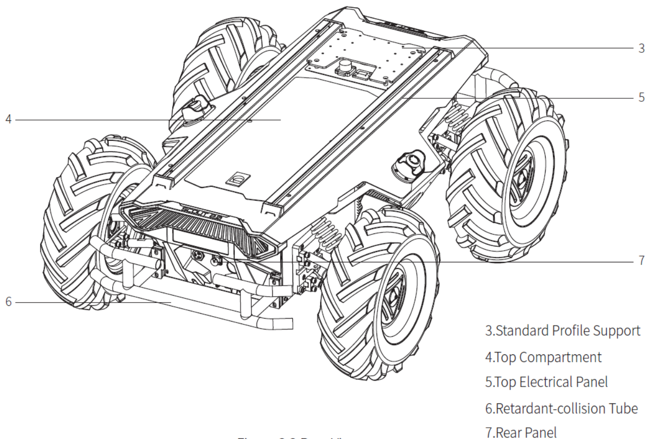
Figure 2.2 Rear View
