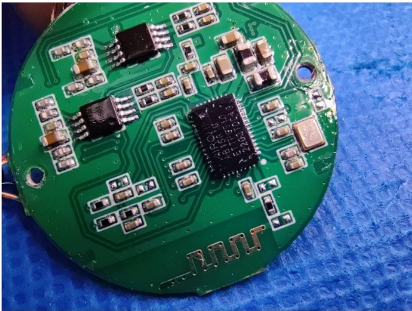
INTERNAL VIEW OF EUT (FIGURE 4)
