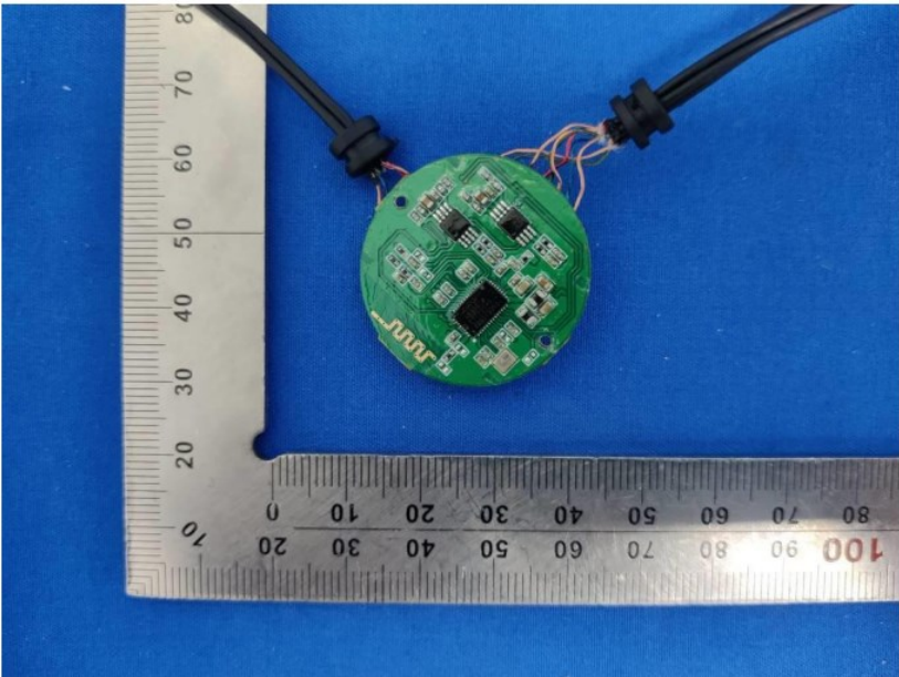
INTERNAL VIEW OF EUT (FIGURE 3)
