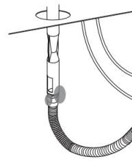
inlet tube / bellows connection (Figure 16)
