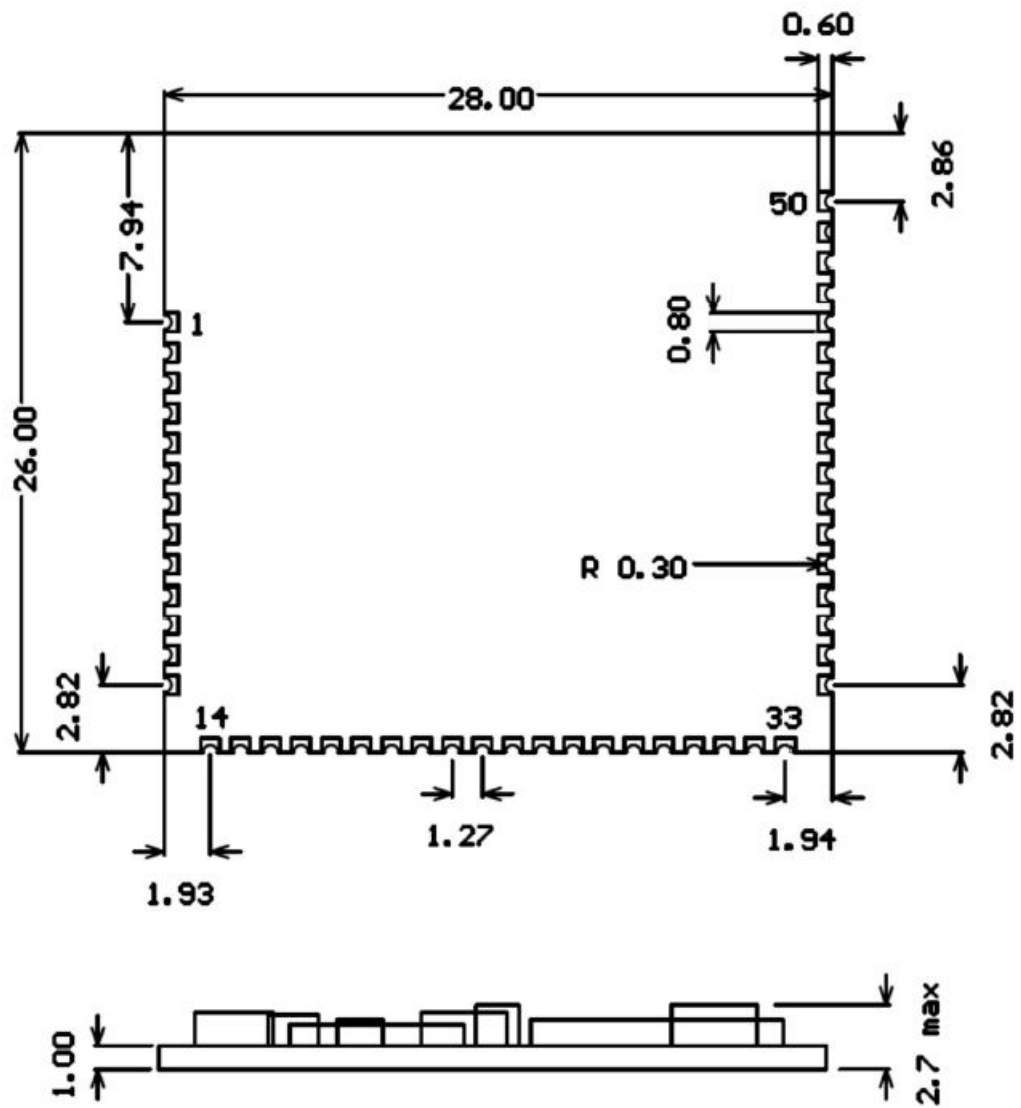
Figure 4 AVT9152 Mechanical Dimensions
