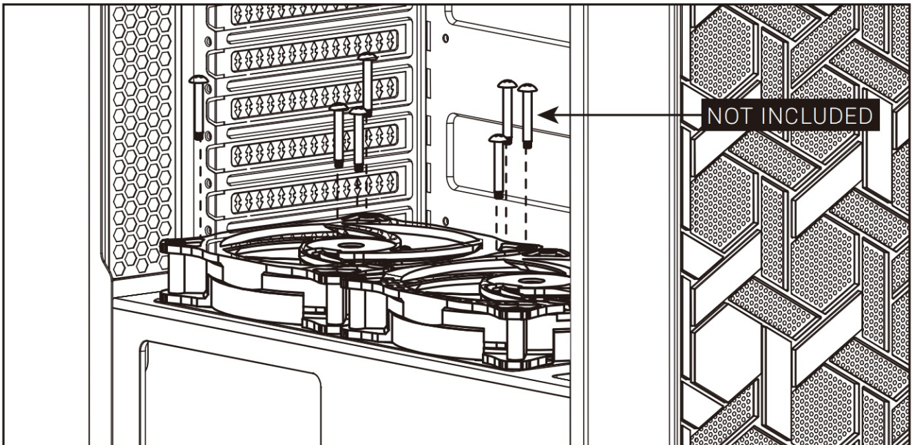
c) Install PSU Fans
