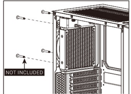
(6c) Install Rear Radiator
