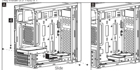
(4a) Install 3.5" HDD x 1
