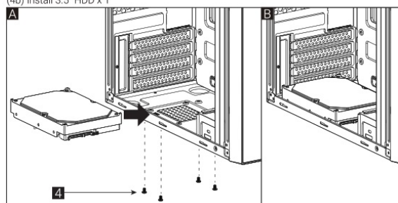
(4b) Install 3.5" HDD x 1
