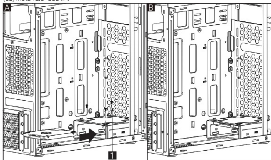
(5a) Install 2.5" SSD x 1
