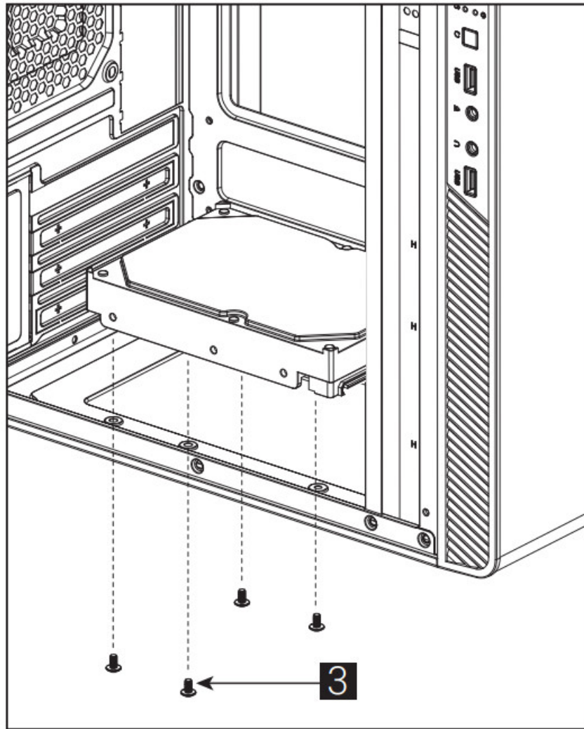
Install 3.5" HDD
