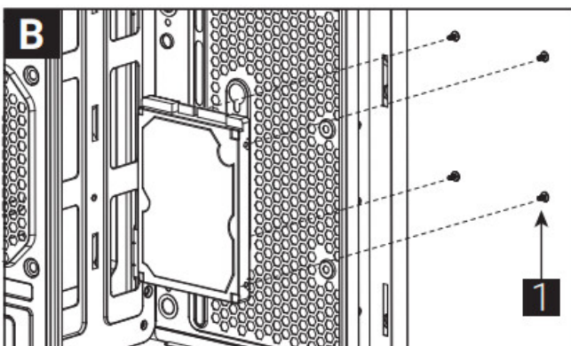
Install 2.5" SSD
