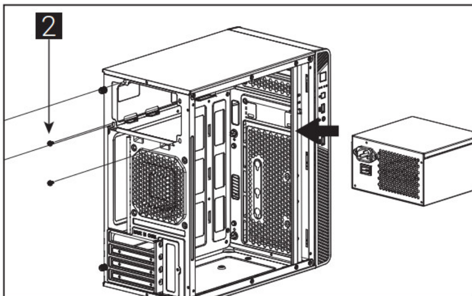
Install PSU
