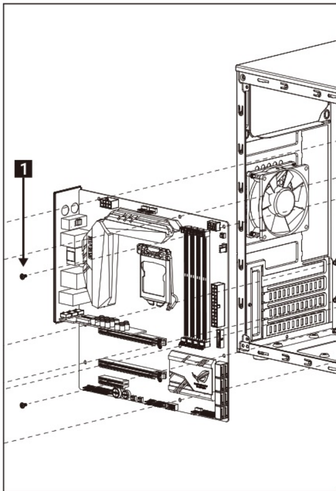
Install Motherboard
