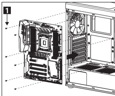
(1) Motherboard
