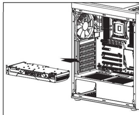
(3) Add-on Card
