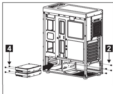
(4) 3.5" HDD x 2
