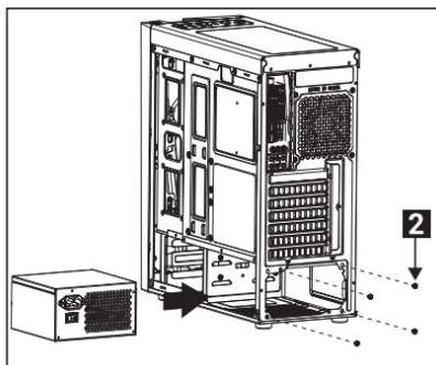
(2) PSU
