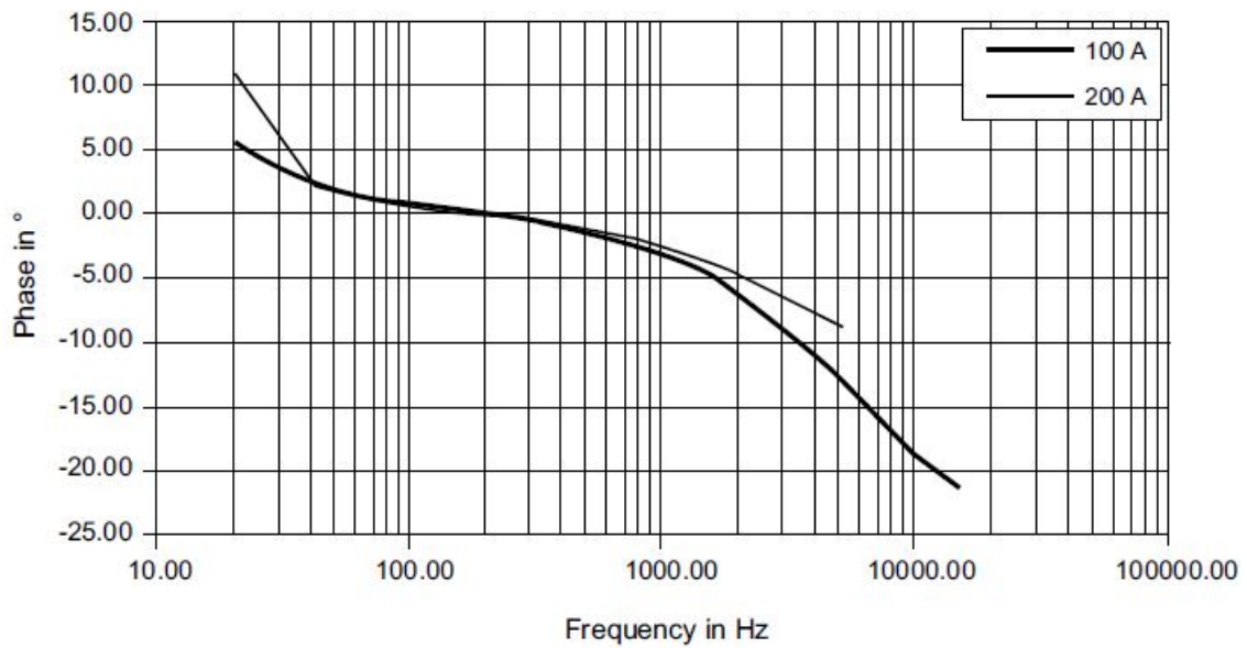
Phase Shift vs. Frequency
