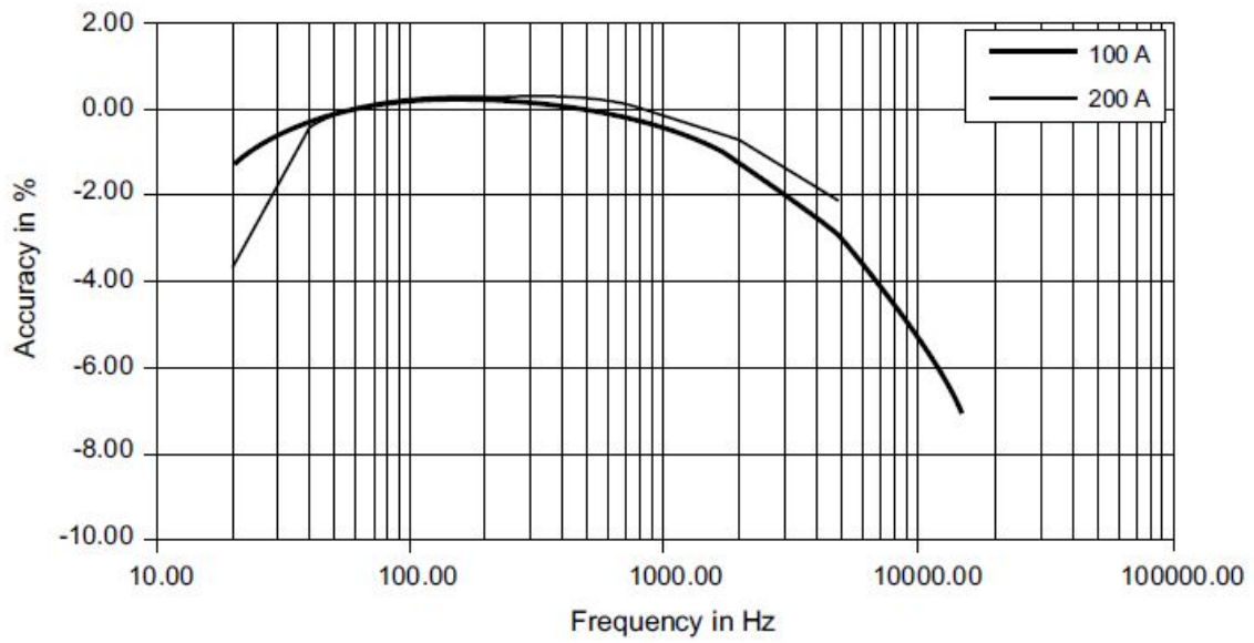
Accuracy vs. Frequency
