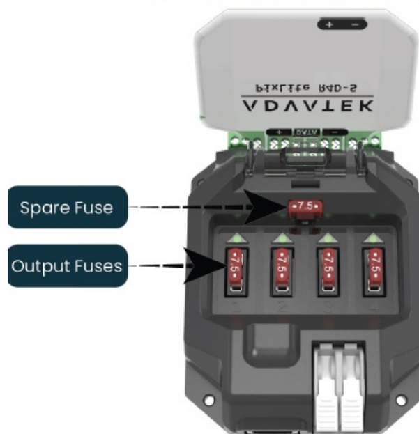
Figure 6: Internal View of the PixLite R4D-S
