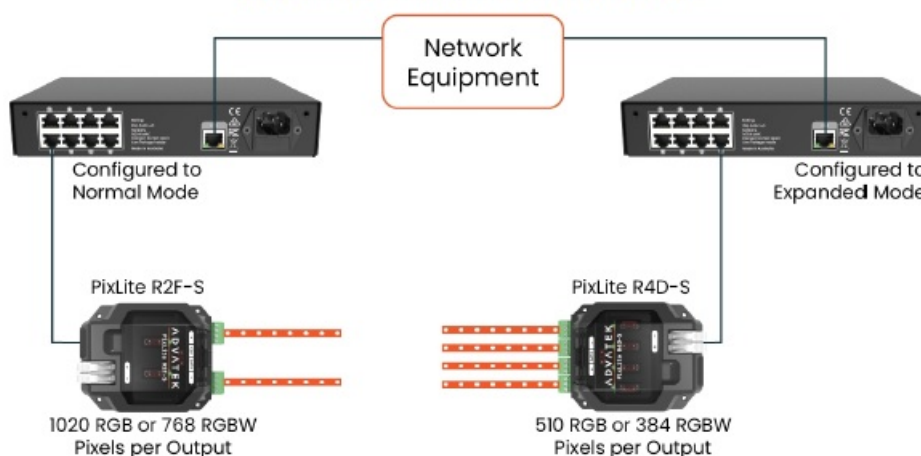
Figure 9: Connecting Receivers to Transmitter
