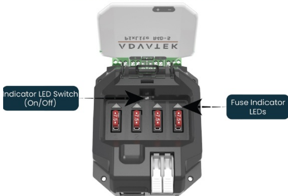
Figure 12: Position of Indicator LEDs and Switch
