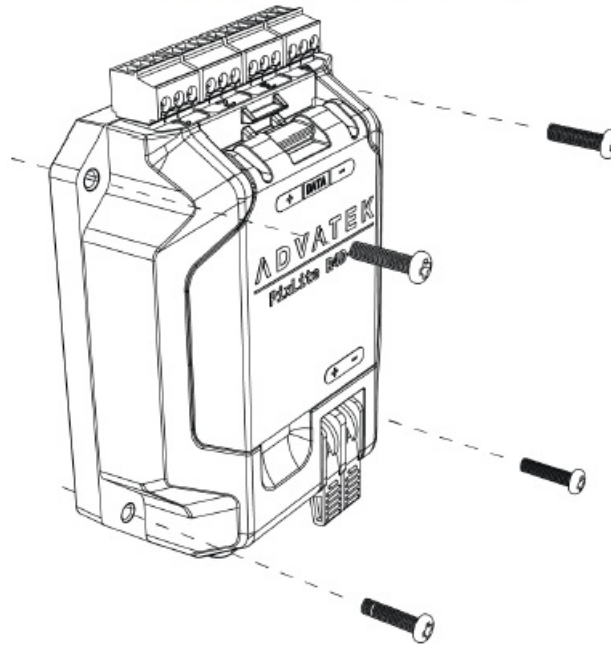
Figure 1: receiver Assembled to Wall
