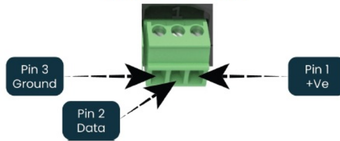
Figure 10: Pixel Output Pinout
