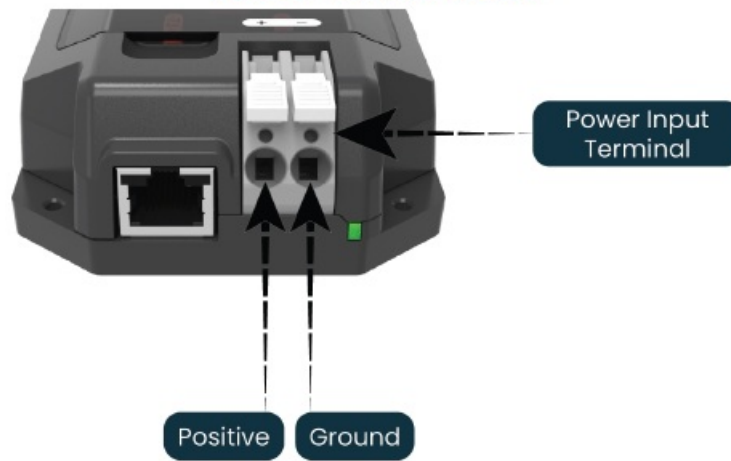
Figure 5: Location of Power Input
