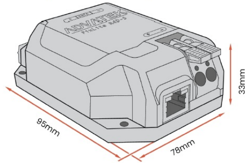
Figure 13: Receiver Mechanical Specifications
