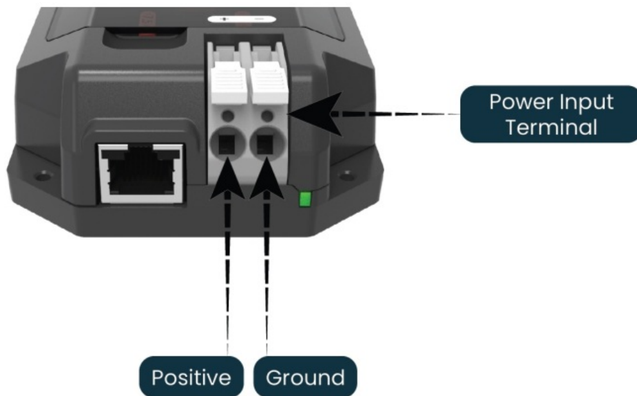
Figure 5: Location of Power Input
