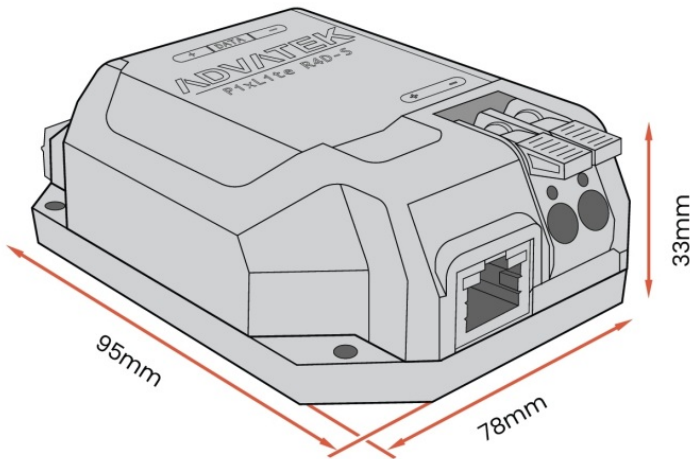
Figure 13: Receiver Mechanical Specifications
