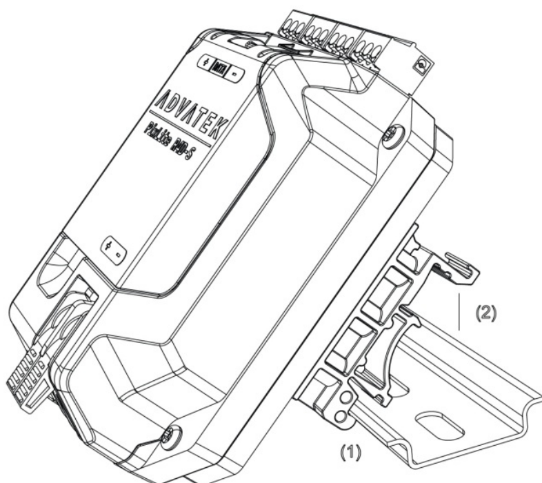
Figure 3: receiver Assembled to DIN Rail
