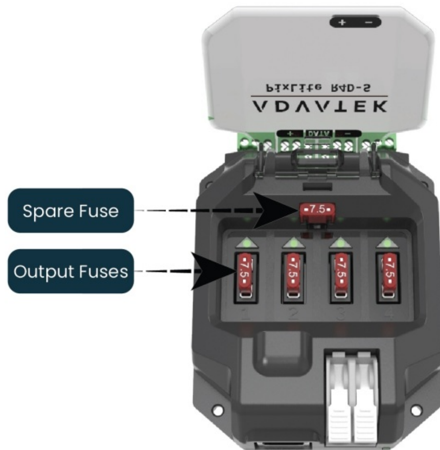
Figure 6: Internal View of the PixLite R4D-S
