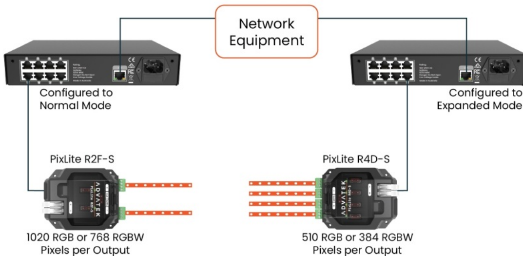
Figure 9: Connecting Receivers to Transmitter
