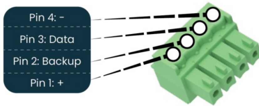
Figure 11: Pixel Output Pinout for Select Backup Pixels
