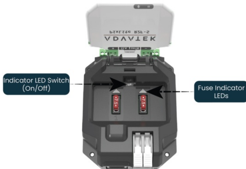
Figure 14: Position of Indicator LEDs and Switch
