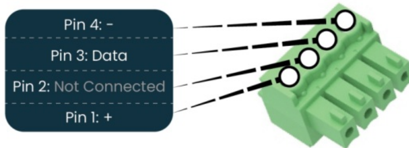
Figure 12: Expanded Mode Pixel Output Pinout
