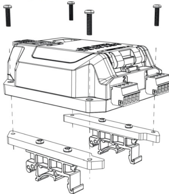
Figure 2: Receiver Assembled to Bracket
