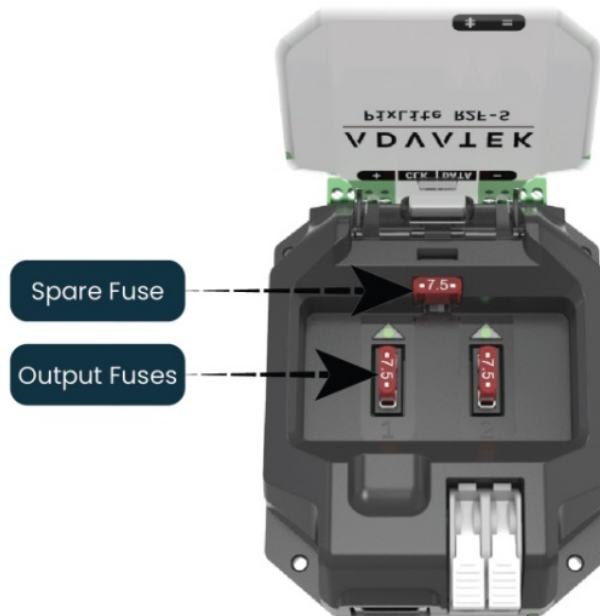
Figure 6: Internal View of the PixLite R2F-S
