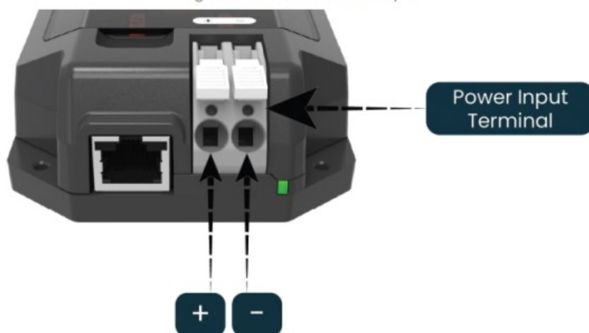
Figure 5: Location of Power Input
