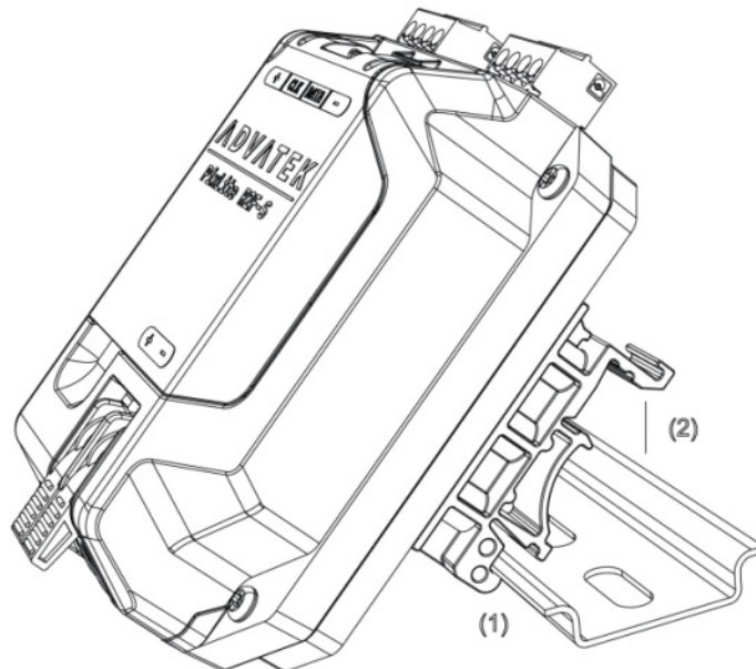
Figure 3: Receiver Assembled to DIN Rail
