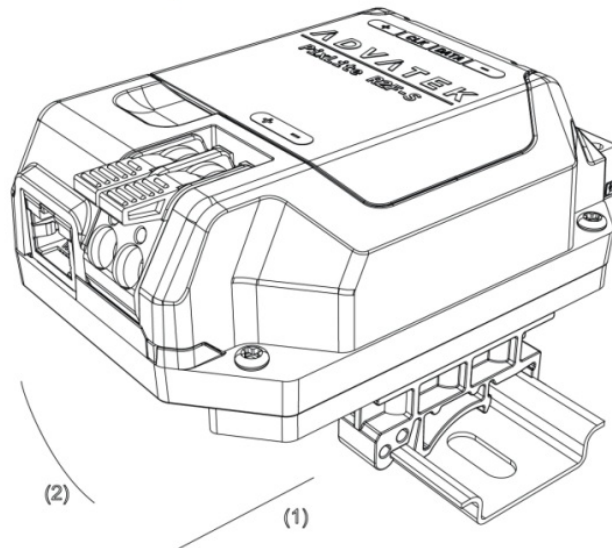
Figure 4: Removal of Receiver from DIN Rail
