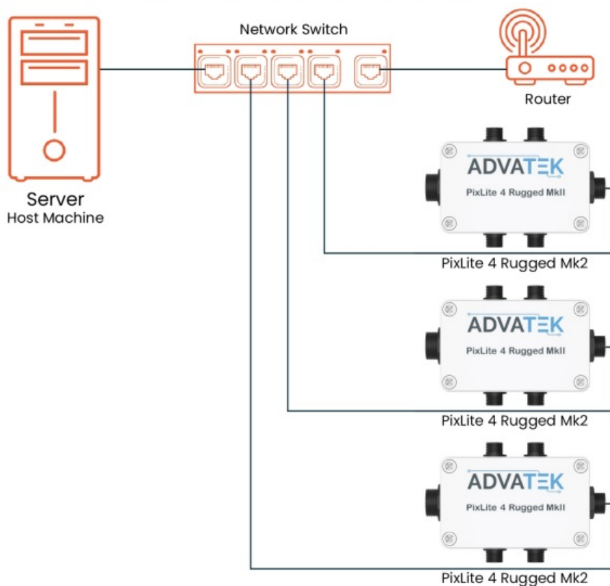
Figure 7: Network Layout using a Server and Switch
