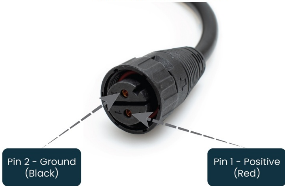
Figure 2: Rugged Power Pigtail Pinout
