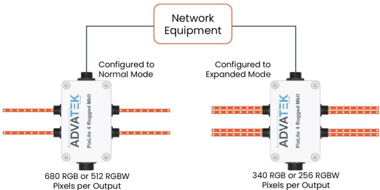
Figure 4: Pixel Set up
