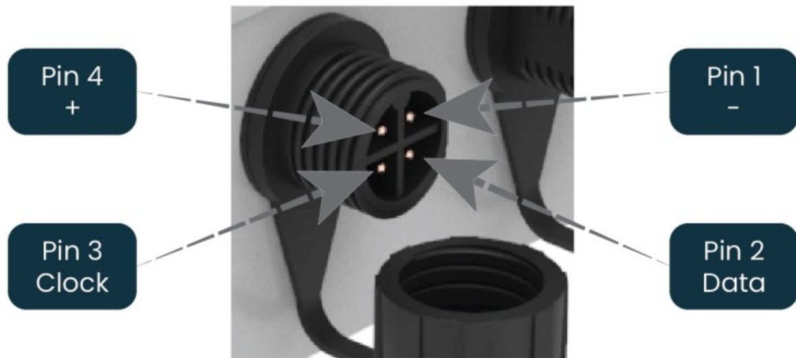
Figure 5: Pixel Output Pinout - Expanded Mode Disabled
