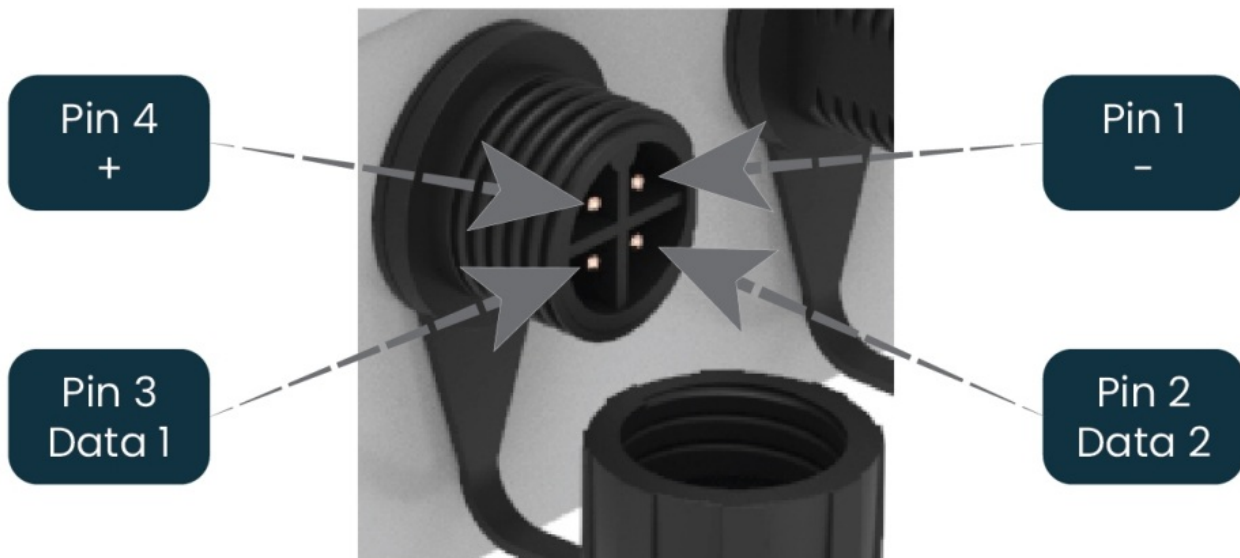
Figure 6: Expanded Mode Pixel Output Pinout
