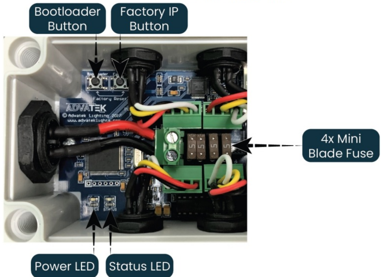
Figure 3: Internal View of the PixLite 4 Rugged Mk2
