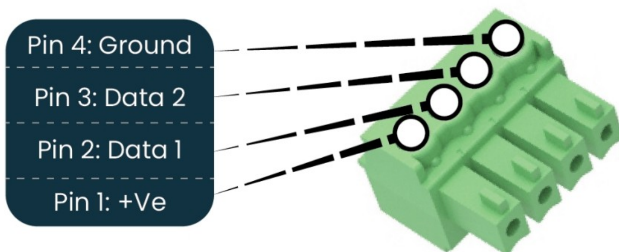
Figure 11: Pixel Output Pinout – Expanded Mode Enabled
