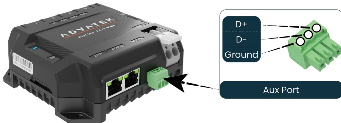
Figure 12: Location and Pinout of the Aux Port
