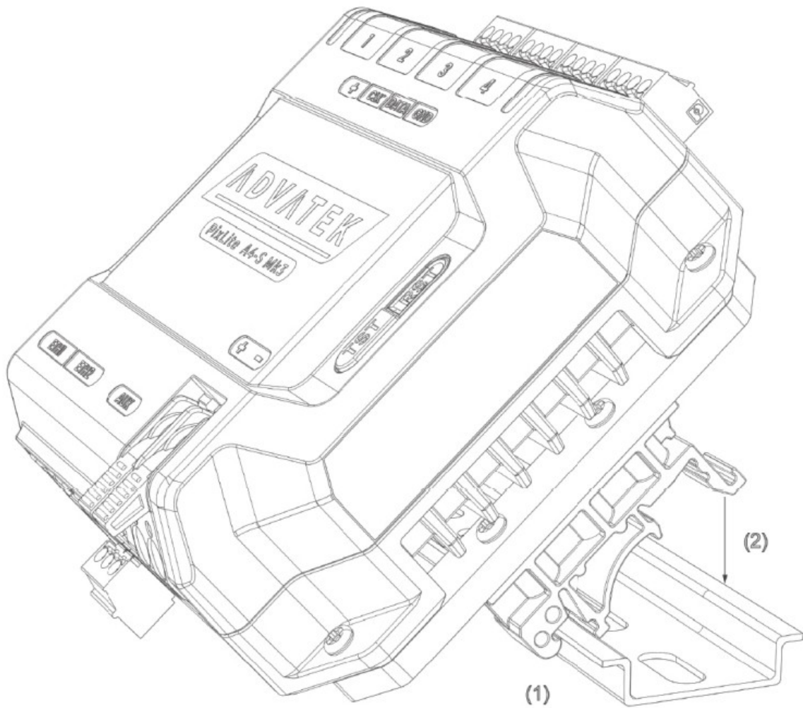
Figure 4: Controller Assembled to DIN Rail
