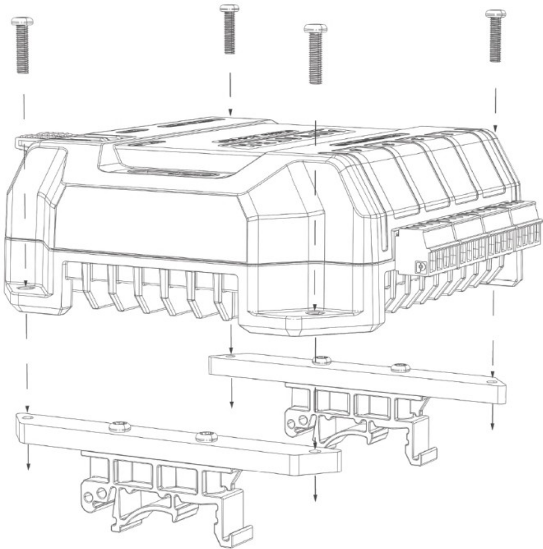
Figure 3: Controller Assembled to Bracket
