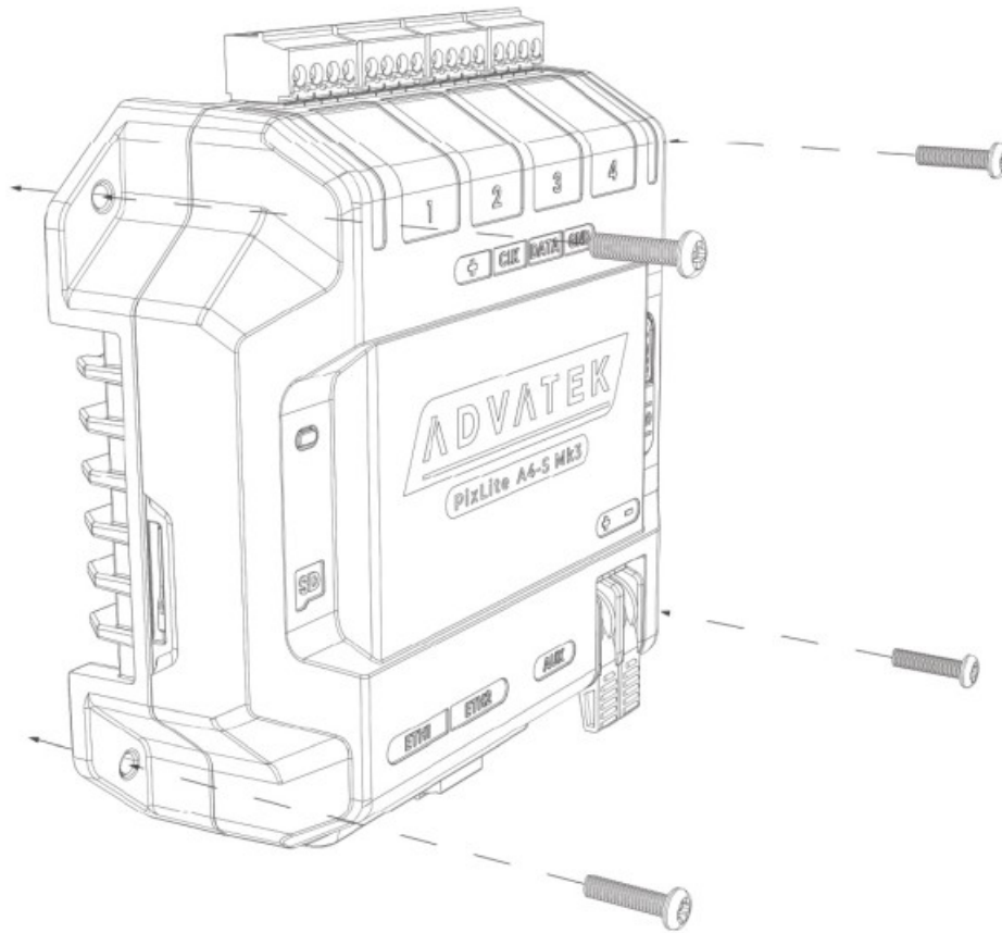
Figure 2: Controller Assembled to Wall
