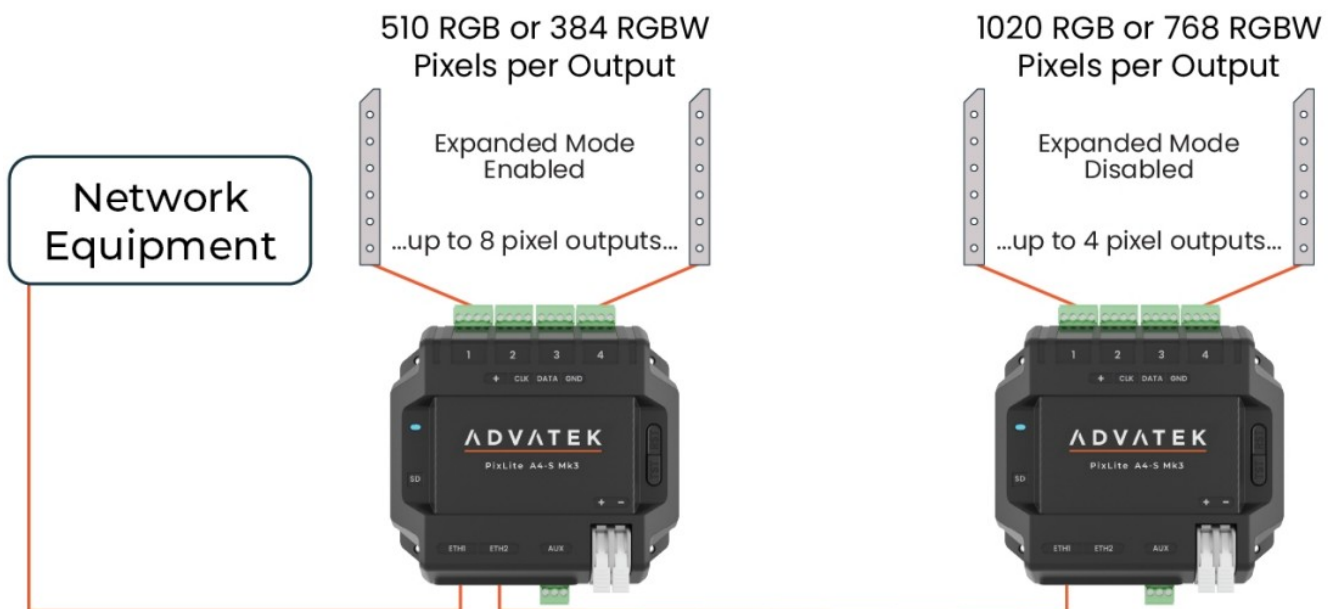
Figure 8: Pixel Set up
