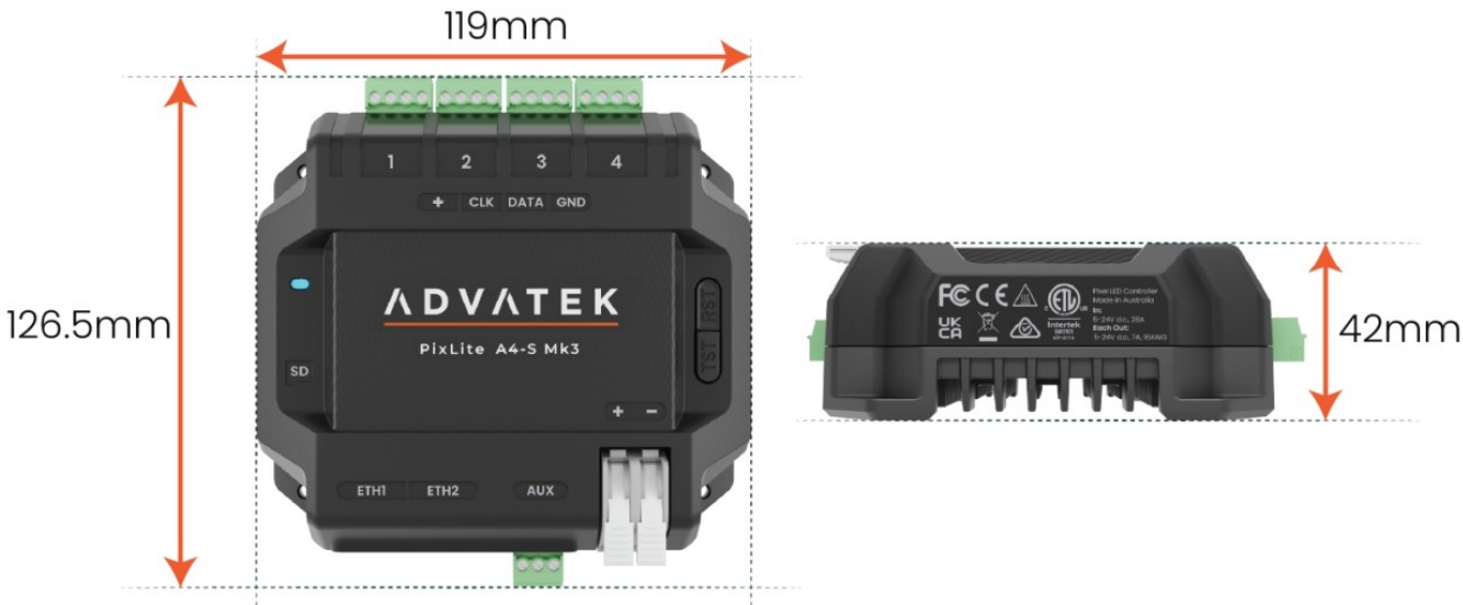
Figure 16: Mechanical Specifications
