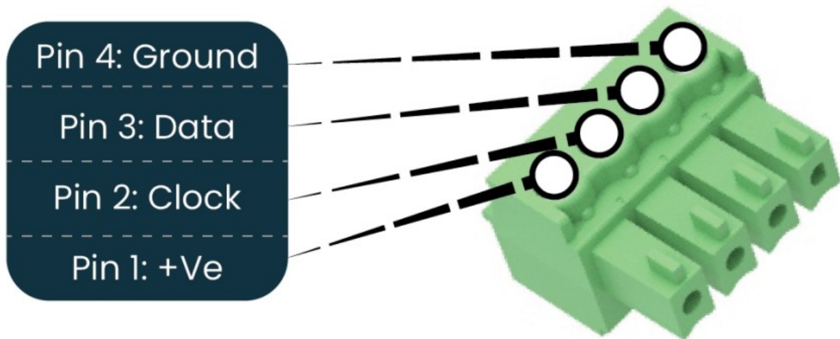
Figure 9: Pixel Output Pinout - Expanded Mode Disabled
