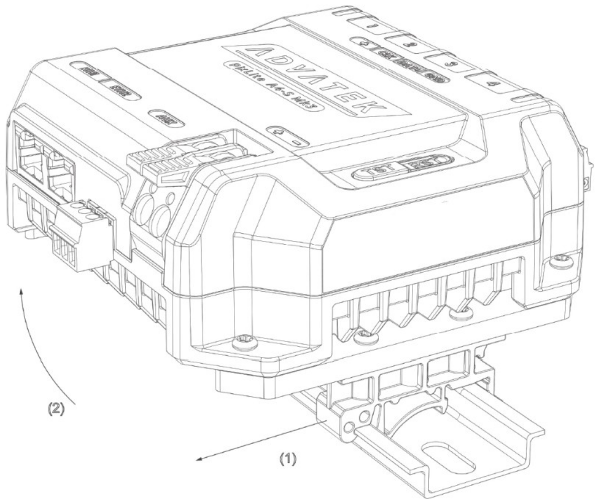
Figure 5: Removal of Controller from DIN Rail
