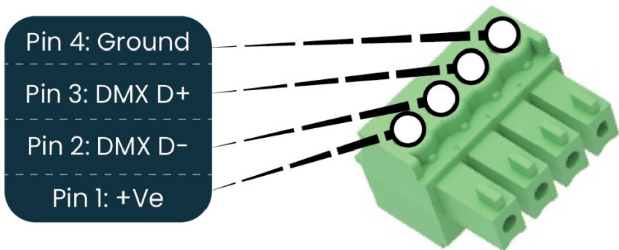
Figure 10: Pixel Output Pinout for Differential DMX512 Pixels
