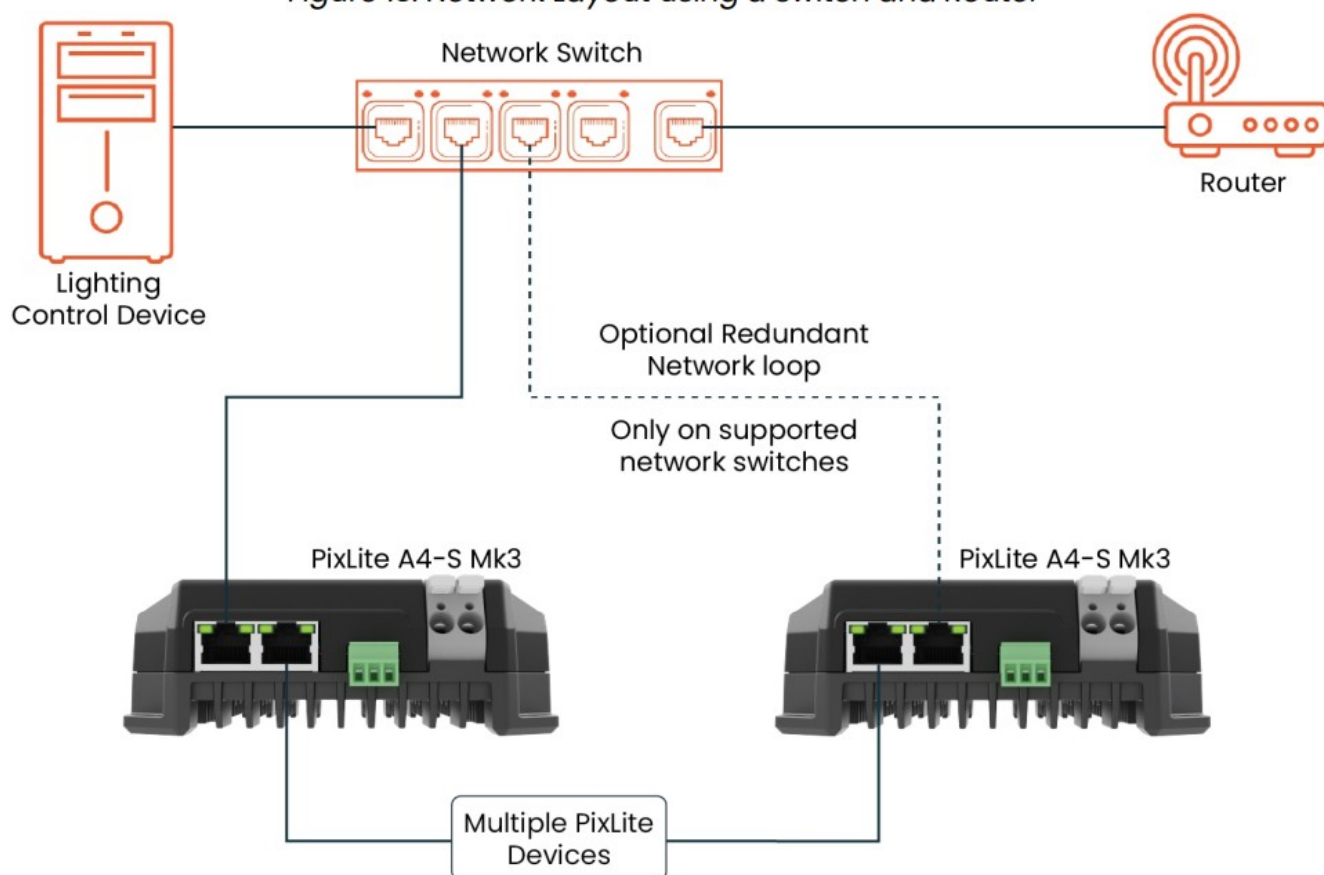
Figure 13: Network Layout using a Switch and Router
