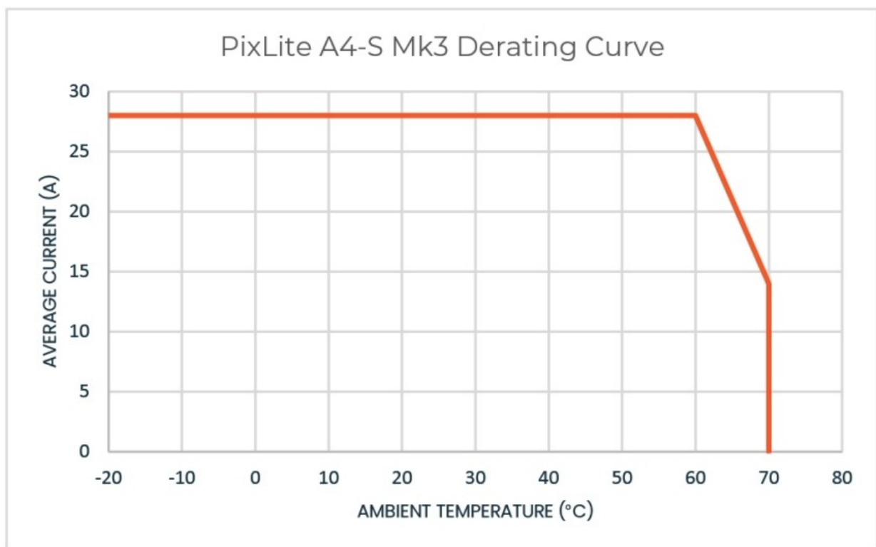
Figure 15: Derating Curve
