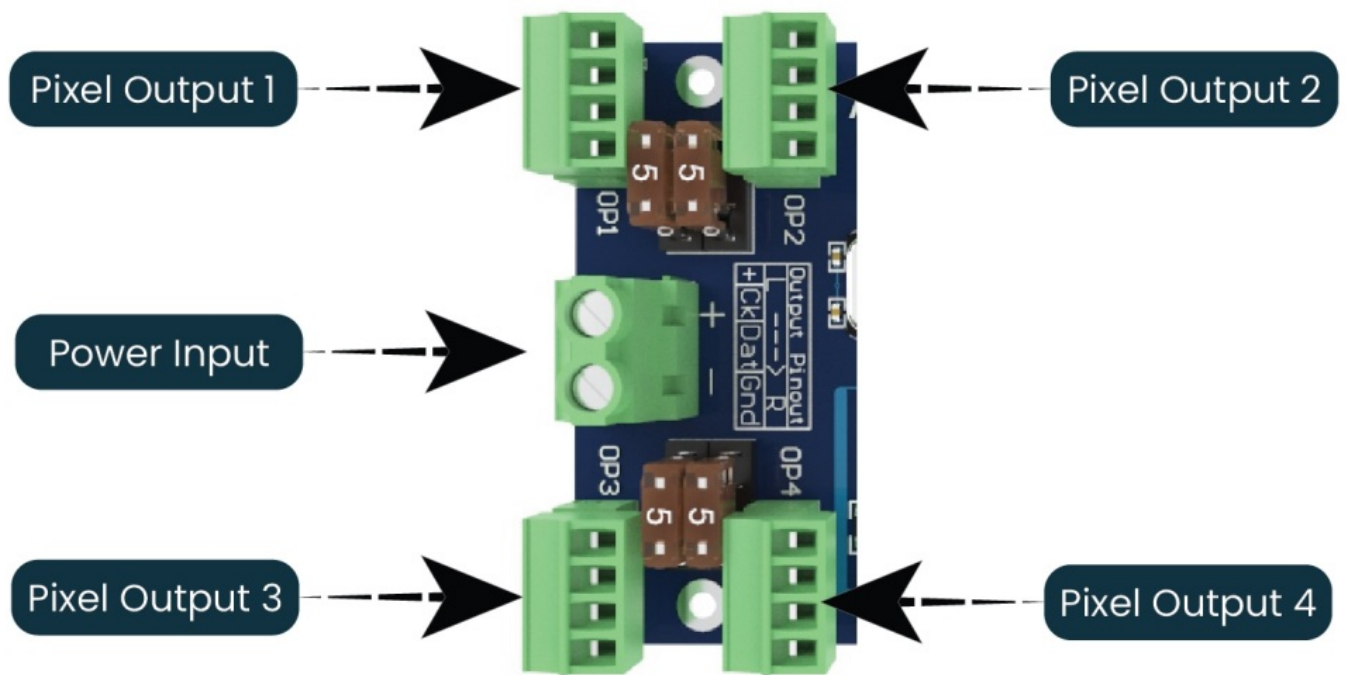
Figure 1: Location of Power Input
