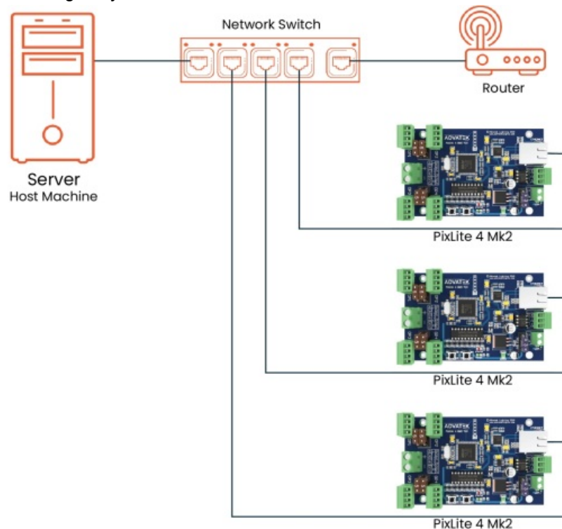
Figure 6: Network Layout using Only a Server
