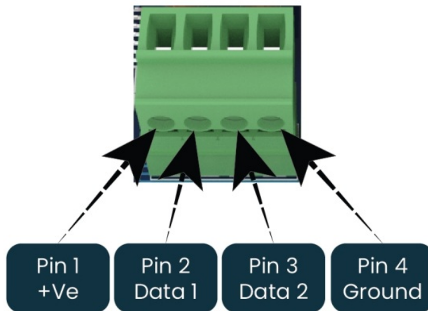
Figure 4: Expanded Mode Pixel Output Pinout
