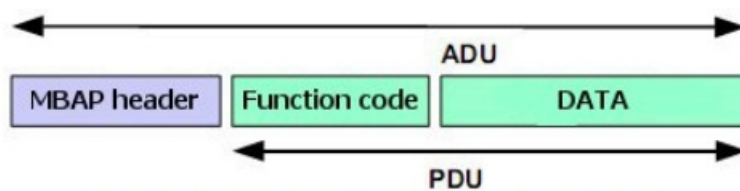
Figure 1: Modbus message on TCP/IP
