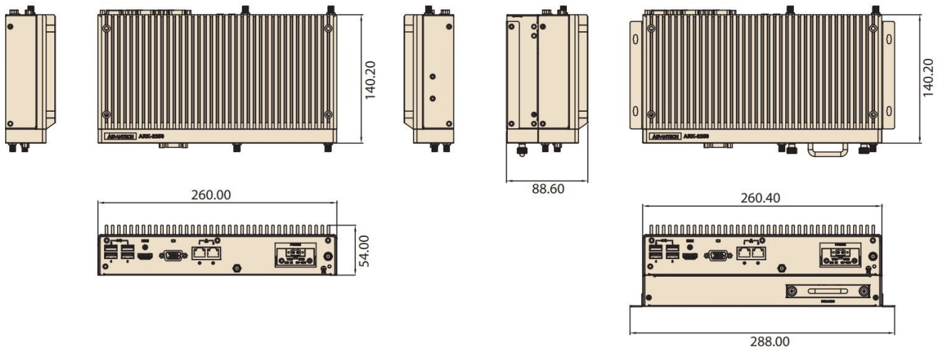
Front Panel External I/O Mechanical Layout/Drawing
