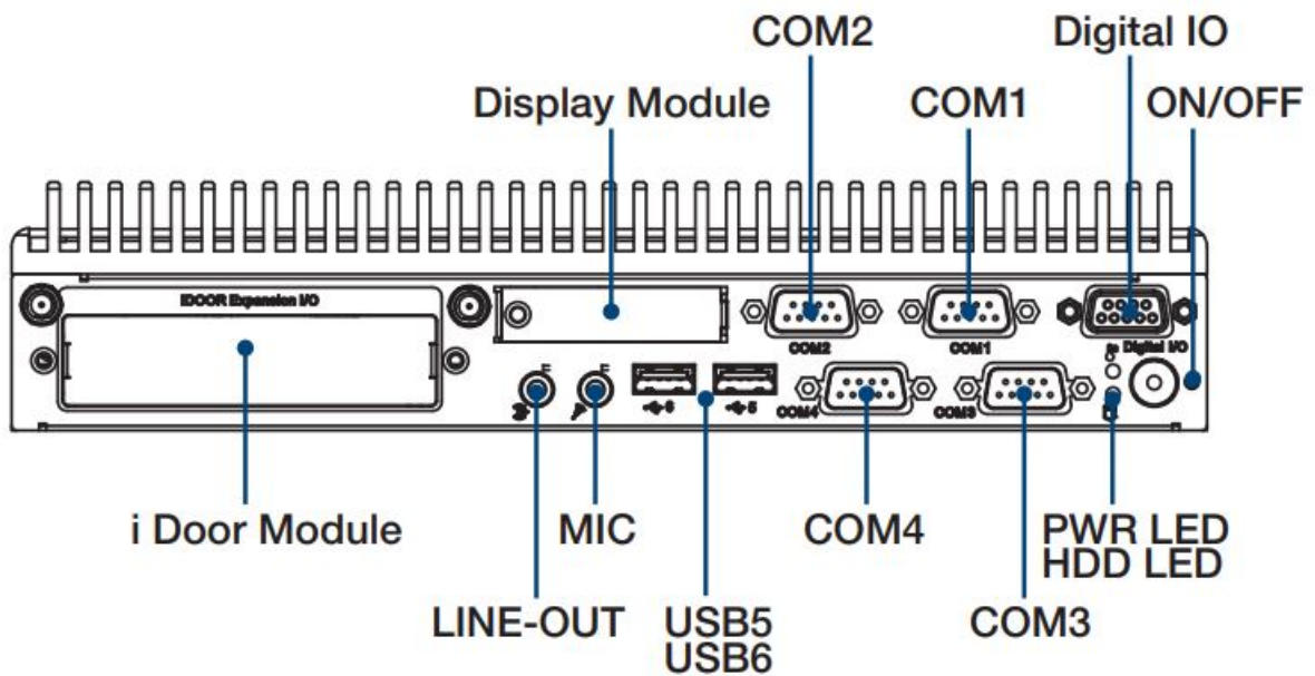
Rear Panel External I/O Mechanical Layout/Drawing
