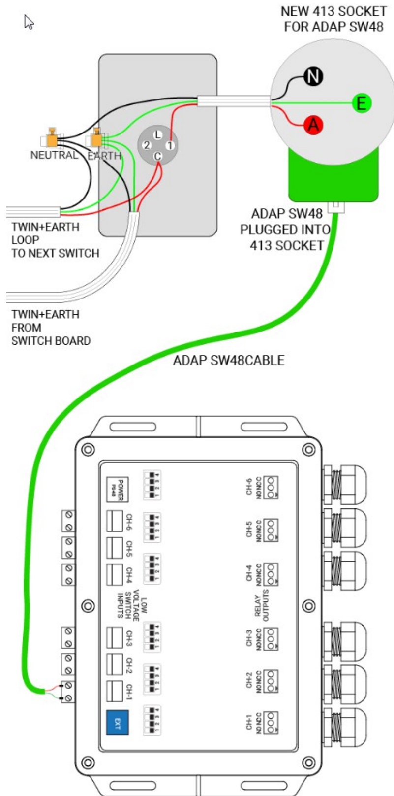
Polarity Sensitive ADAP 48SWCABLE10/20
