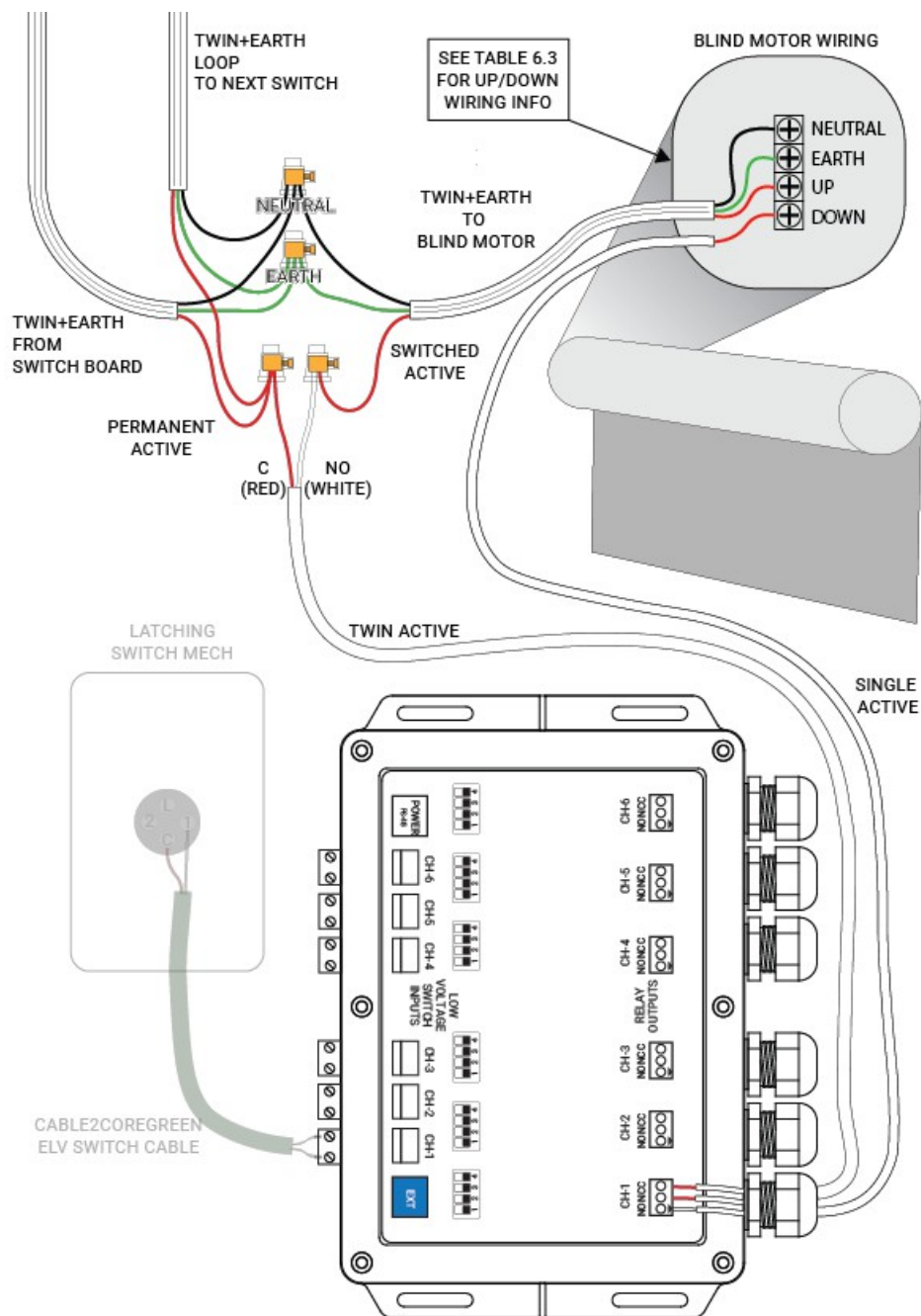
Roller Blind Wiring – Method 2 (using 240V switching [using ADAP SW48] on inputs)
