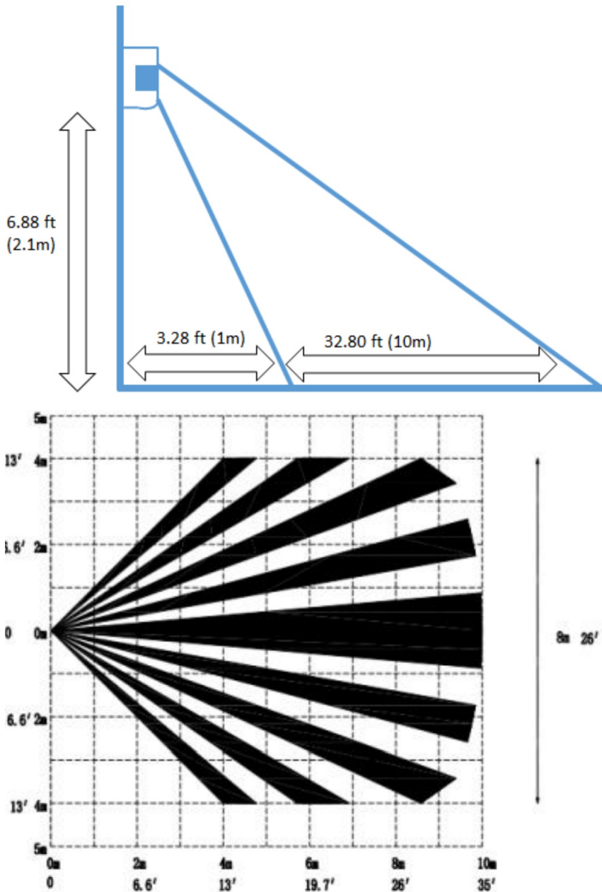
Figure 3: Sensor range and detection
